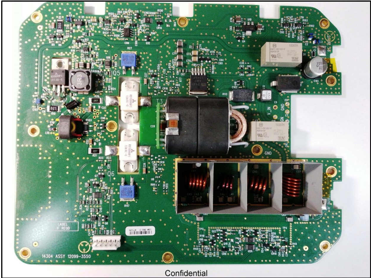
Photograph 13: PCB Top View - Filter Assembly
