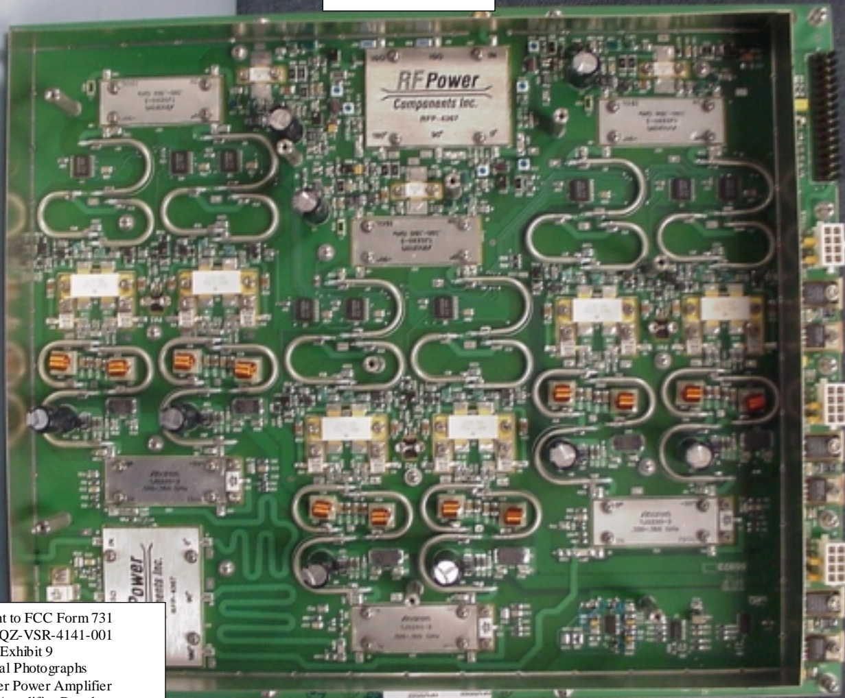
Power Amplifier Board
