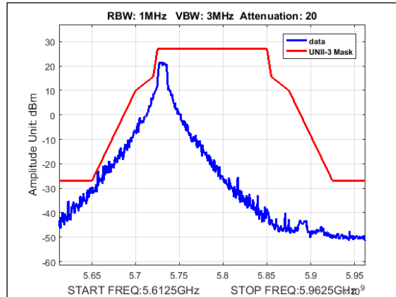
Plot 398. Undesirable Emissions, UNII-3 Emissions Mask, 5M, 5730MHz, 80mni
