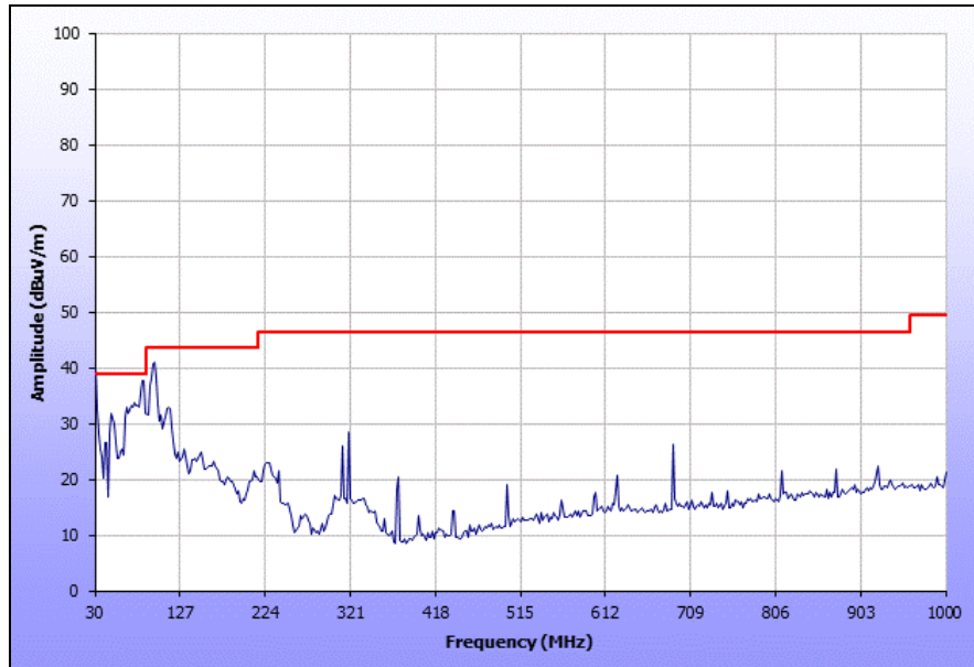
Plot 397. Undesirable Emissions 30MHz – 1GHz (Worst case)
