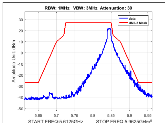
Plot 405. Undesirable Emissions, UNII-3 Emissions Mask, 5M, 5845MHz, 8Omni
