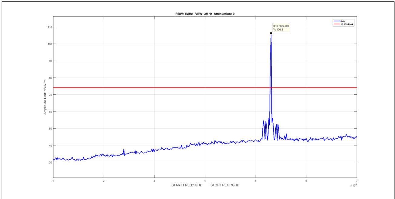
Plot 887. Undesirable Emissions, 50mni, Peak, 1-7GHz, 5M, 5300, pow8
