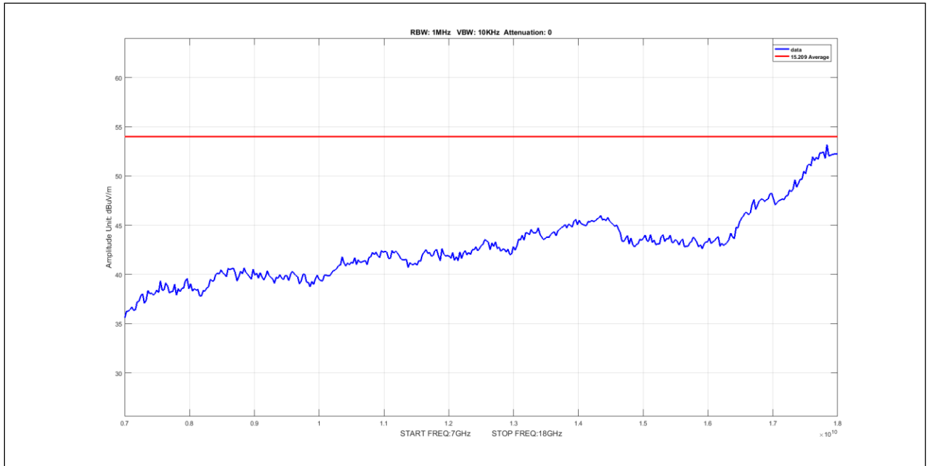
Plot 882. Undesirable Emissions, 5Omni, Average, 7-18GHz, 40M, 5330, pow4
