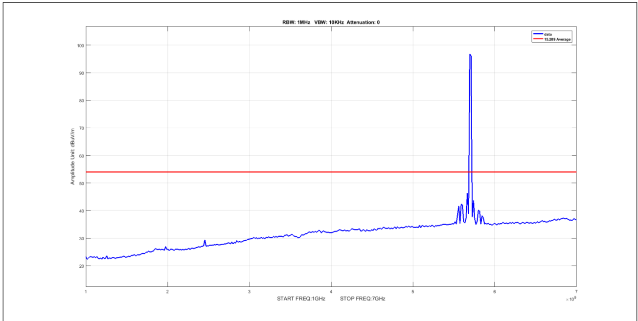
Plot 939. Undesirable Emissions, 80mni, Average, 1-7GHz, 5M, 5700, pow6
