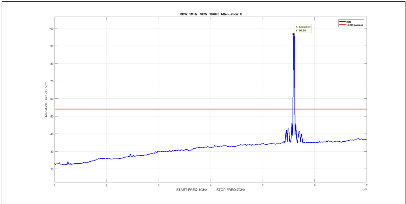
Plot 938. Undesirable Emissions, 80mni, Average, 1-7GHz, 5M, 5595, pow6
