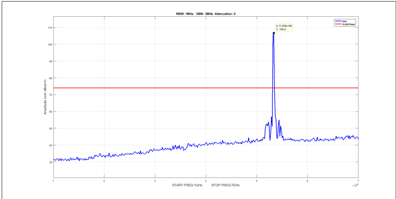
Plot 894. Undesirable Emissions, 5Omni, Peak, 1-7GHz, 10M, 5330, pow11
