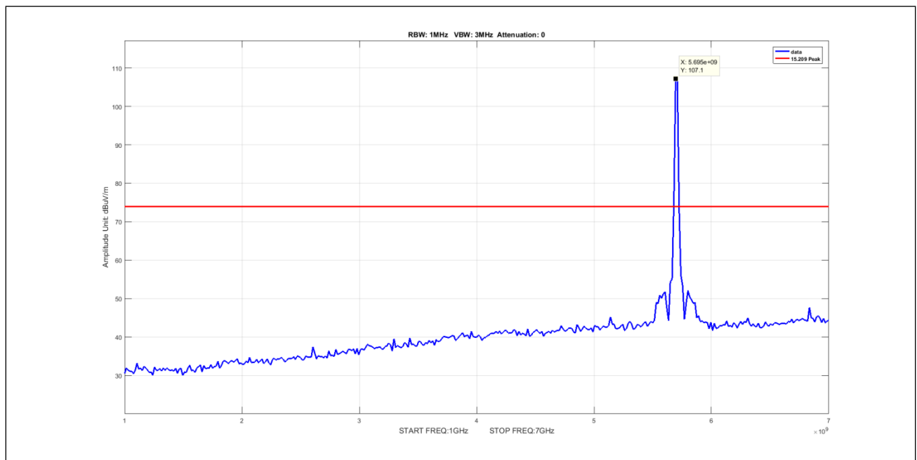
Plot 903. Undesirable Emissions, 50mni, Peak, 1-7GHz, 20M, 5700, pow11
