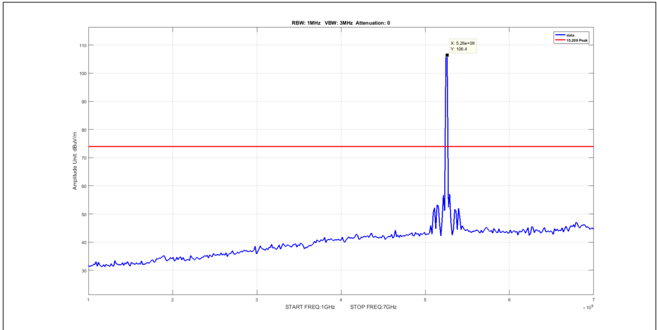
Plot 886. Undesirable Emissions, 50mni, Peak, 1-7GHz, 5M, 5252.5, pow8
