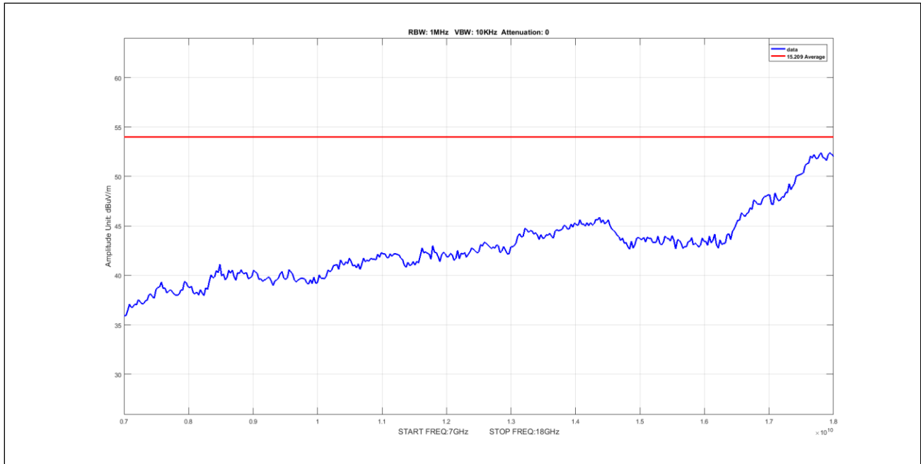
Plot 884. Undesirable Emissions, 5Omni, Average, 7-18GHz, 40M, 5595, pow19
