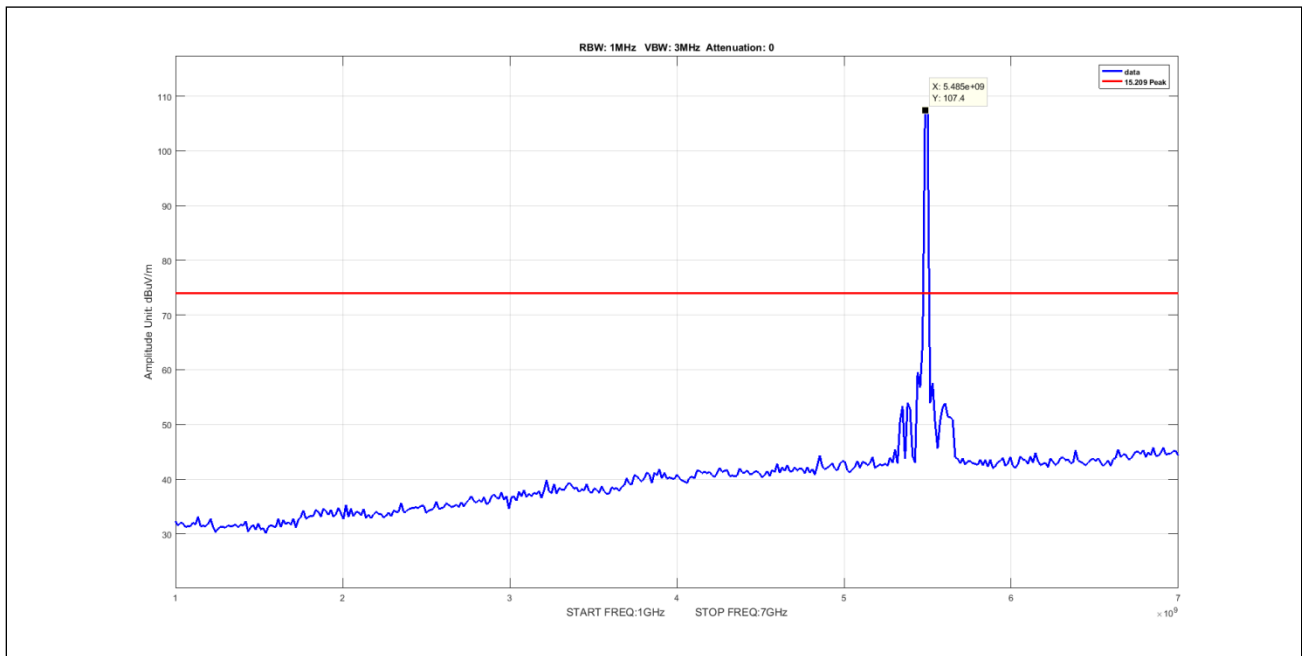
Plot 895. Undesirable Emissions, 5Omni, Peak, 1-7GHz, 10M, 5490, pow12
