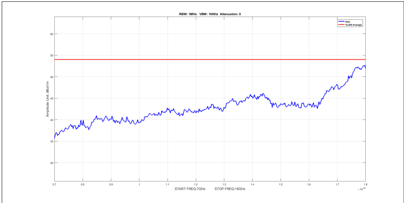
Plot 885. Undesirable Emissions, 5Omni, Average, 7-18GHz, 40M, 5700, pow7
