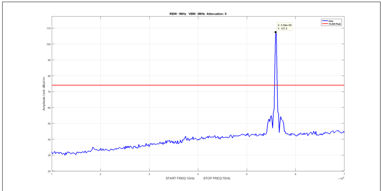
Plot 902. Undesirable Emissions, 50mni, Peak, 1-7GHz, 20M, 5595, pow14
