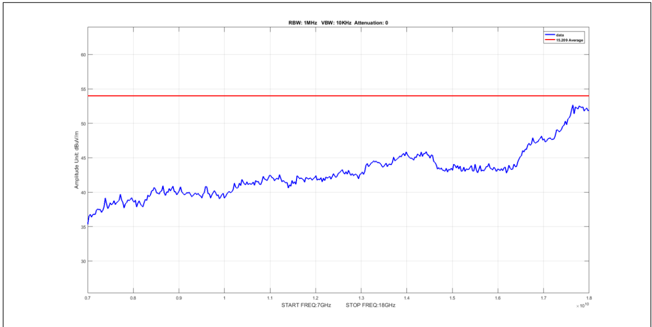
Plot 883. Undesirable Emissions, 5Omni, Average, 7-18GHz, 40M, 5490, pow4
