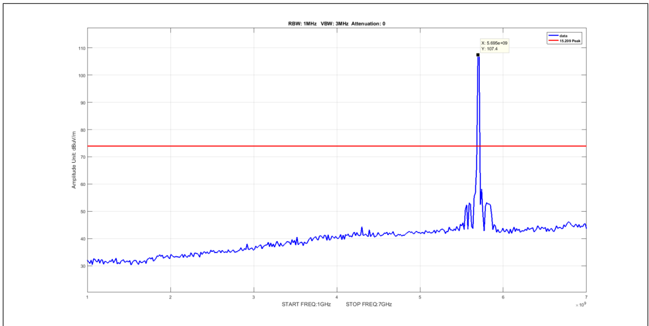
Plot 897. Undesirable Emissions, 5Omni, Peak, 1-7GHz, 10M, 5700, pow11
