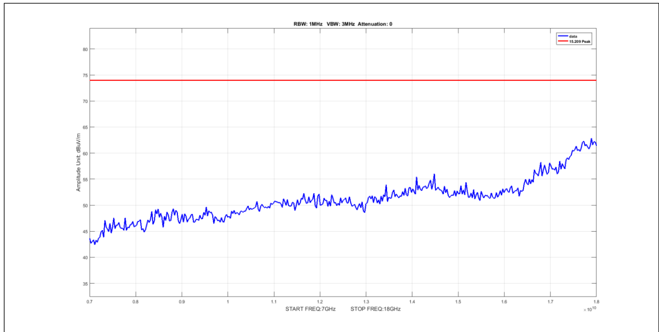
Plot 928. Undesirable Emissions, 50mni, Peak, 7-18GHz, 40M, 5270, pow19
