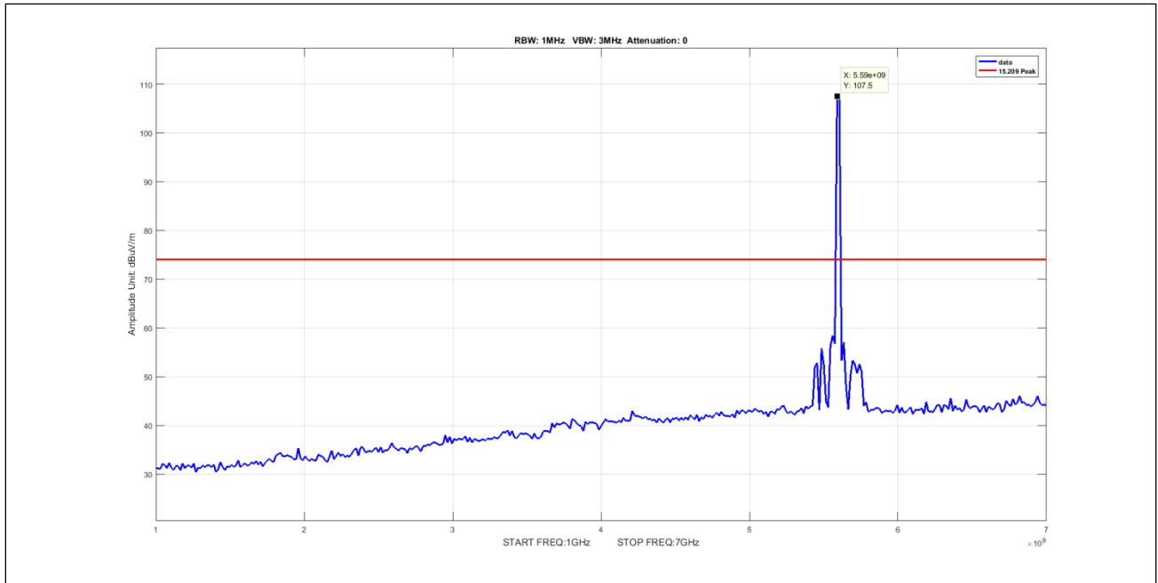
Plot 896. Undesirable Emissions, 5Omni, Peak, 1-7GHz, 10M, 5595, pow11
