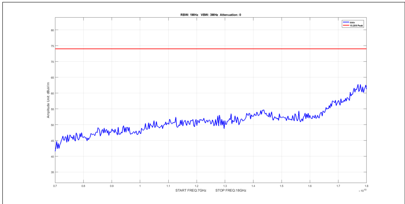
Plot 929. Undesirable Emissions, 50mni, Peak, 7-18GHz, 40M, 5300, pow19
