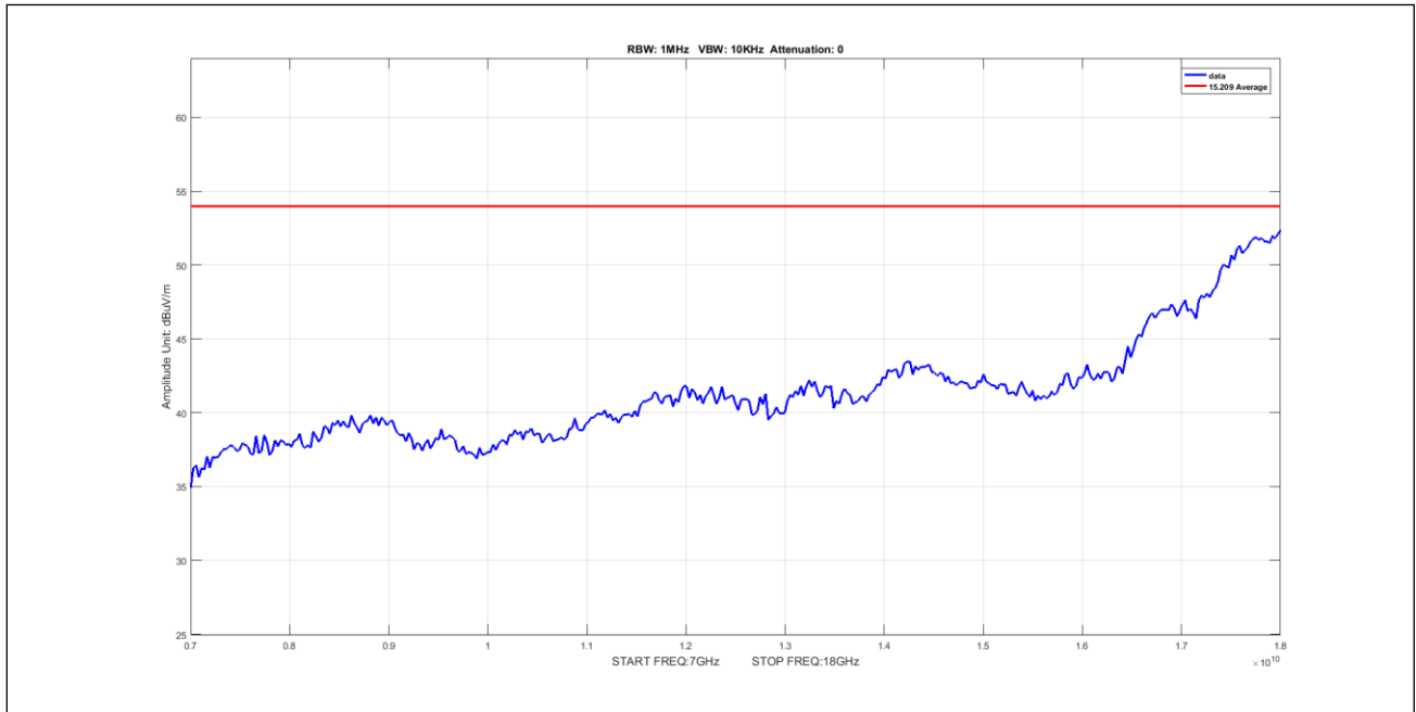
Plot 531. Undesirable Emissions, 5Omni Avg 7-18GHz 20M 5240 pow20
