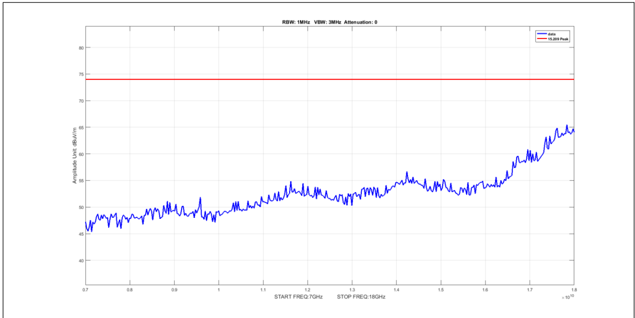
Plot 550. Undesirable Emissions, 50mV Peak 7-18GHz 10M 5170 pow17
