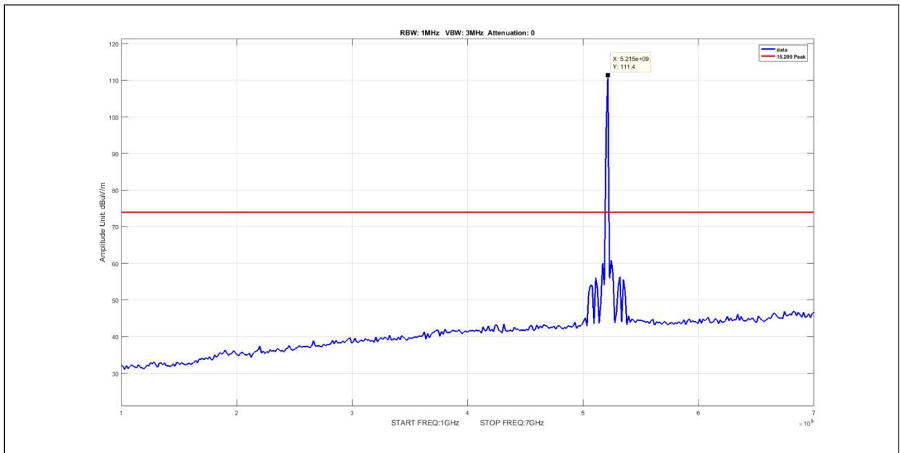
Plot 536. Undesirable Emissions, 50mni Peak 1-7GHz 5M 5210 pow14
