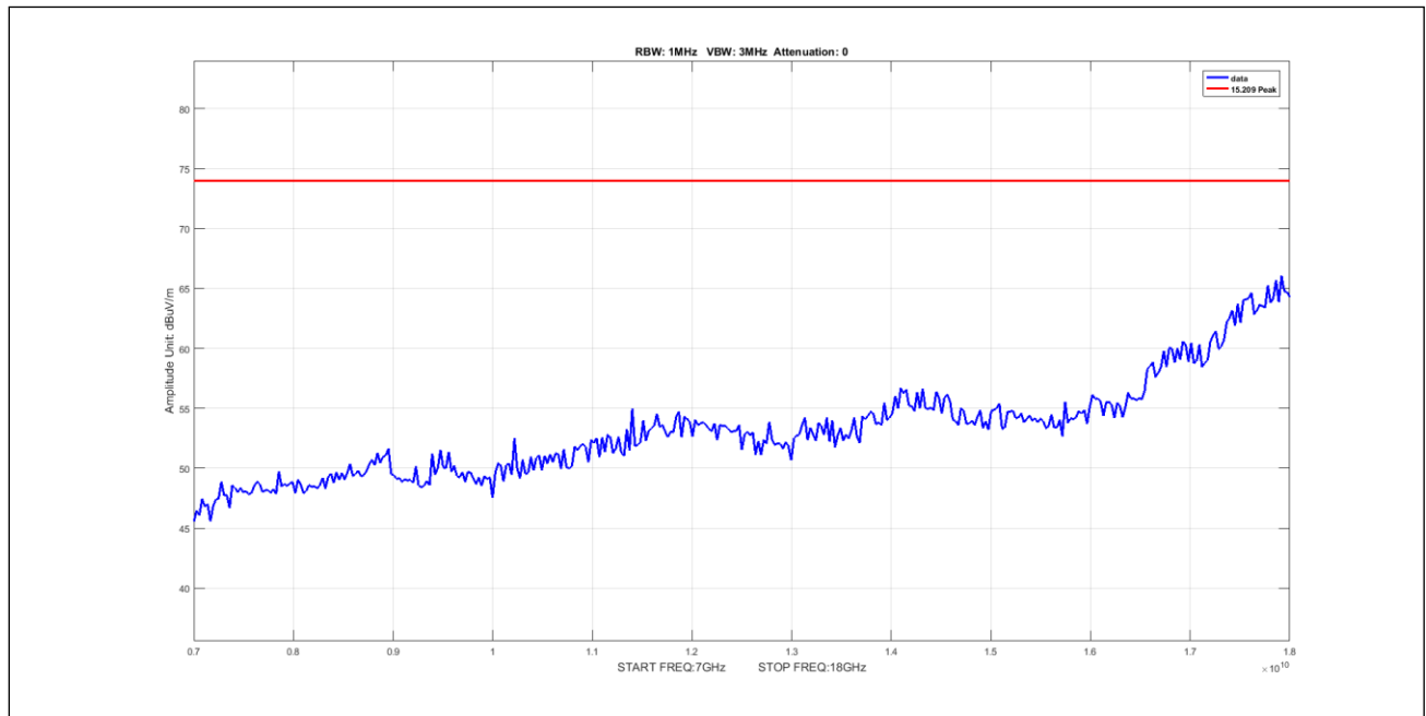
Plot 547. Undesirable Emissions, 5Omni Peak 7-18GHz 5M 5170 pow14
