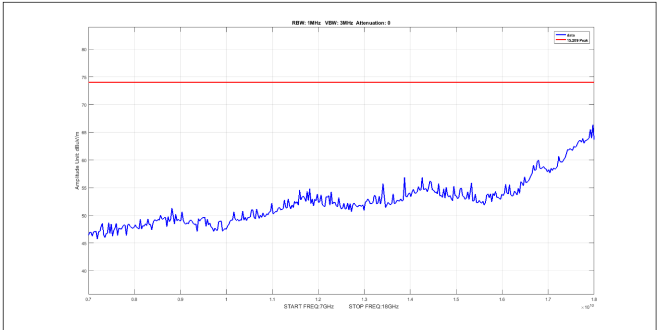
Plot 549. Undesirable Emissions, 50mV Peak 7-18GHz 5M 5247.5 pow14
