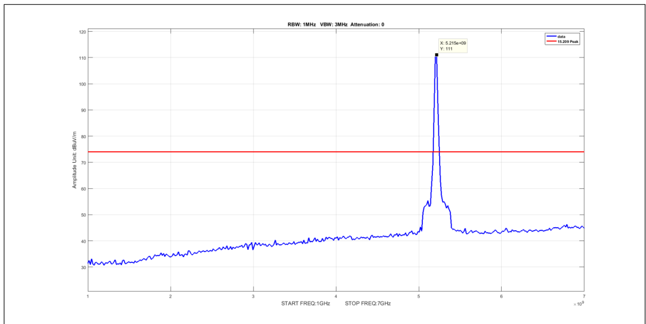
Plot 542. Undesirable Emissions, 5Omni Peak 1-7GHz 20M 5210 pow19
