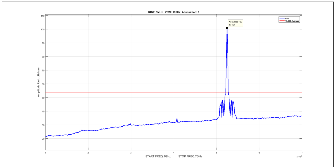
Plot 514. Undesirable Emissions, 50mni Avg 1-7GHz 10M 5245 pow17
