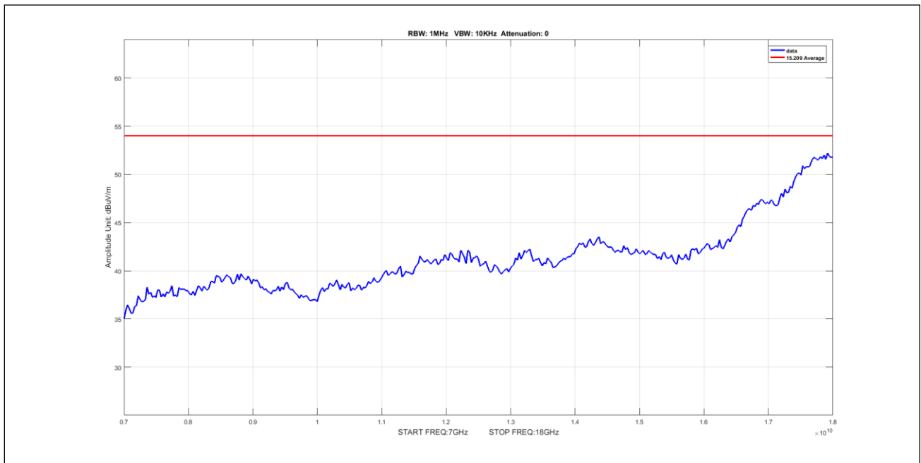
Plot 532. Undesirable Emissions, 5Omni Avg 7-18GHz 40M 5170 pow3
