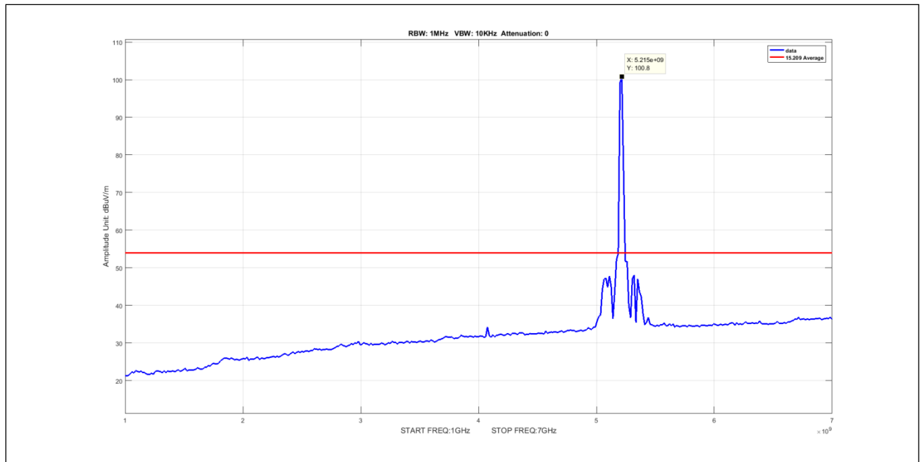
Plot 513. Undesirable Emissions, 50mni Avg 1-7GHz 10M 5210 pow17
