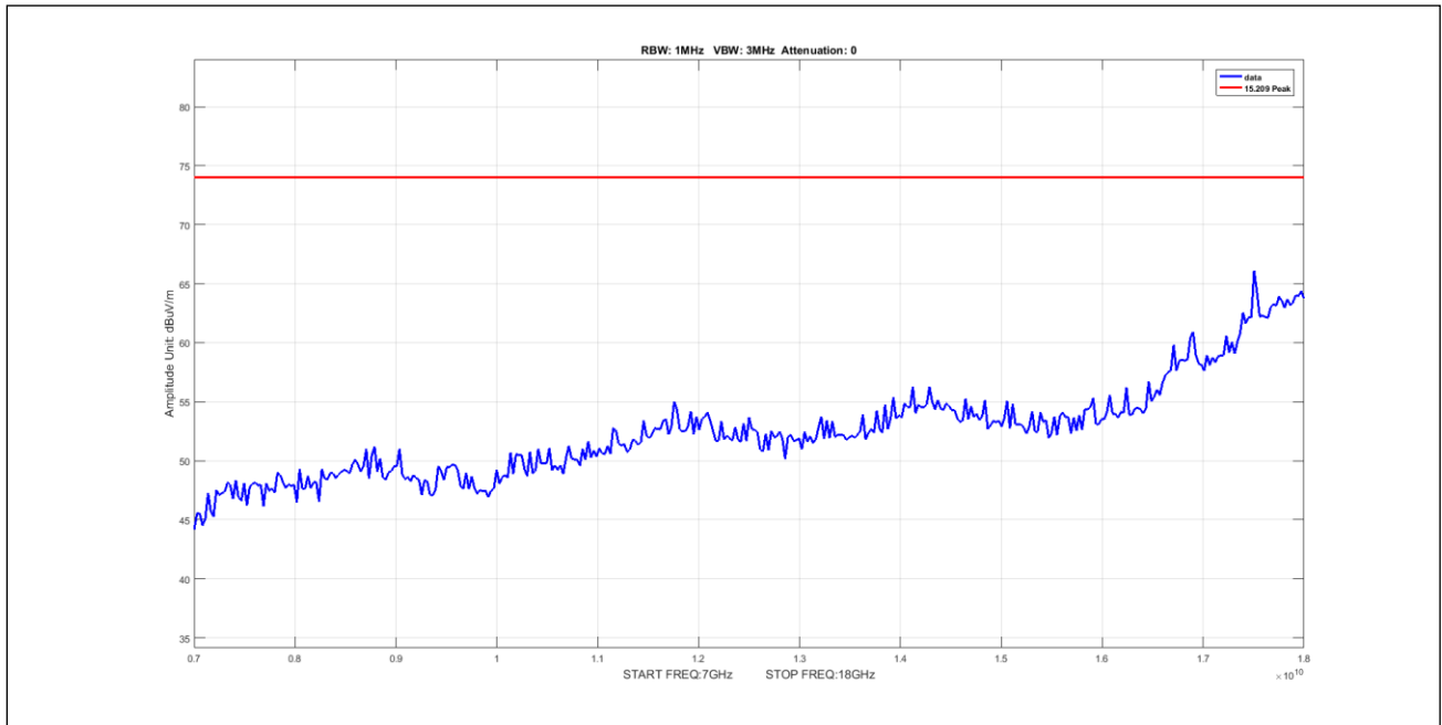
Plot 552. Undesirable Emissions, 50mni Peak 7-18GHz 10M 5245 pow17
