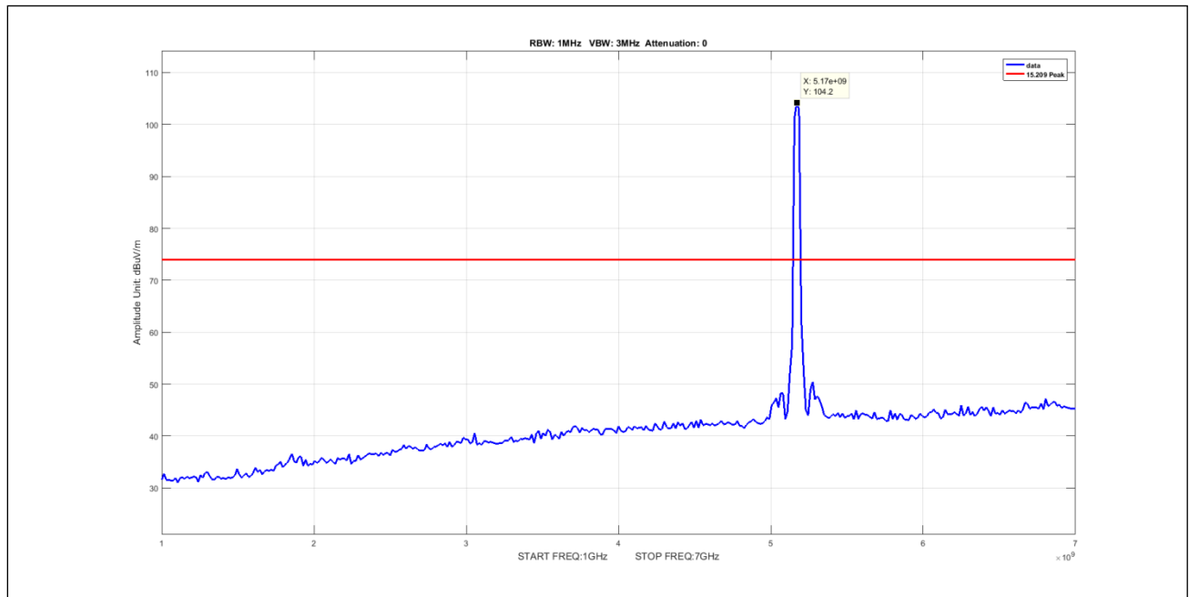
Plot 541. Undesirable Emissions, 5Omni Peak 1-7GHz 20M 5170 pow10
