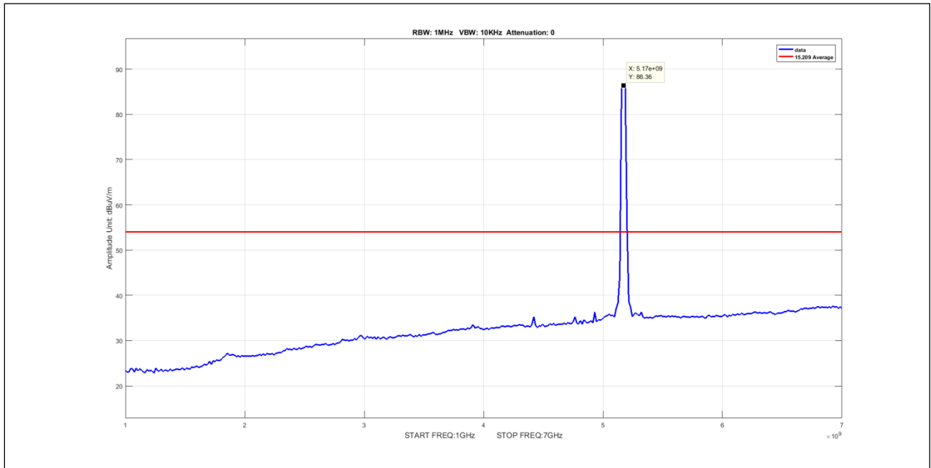
Plot 518. Undesirable Emissions, 5Omni Avg 1-7GHz 40M 5170 pow3
