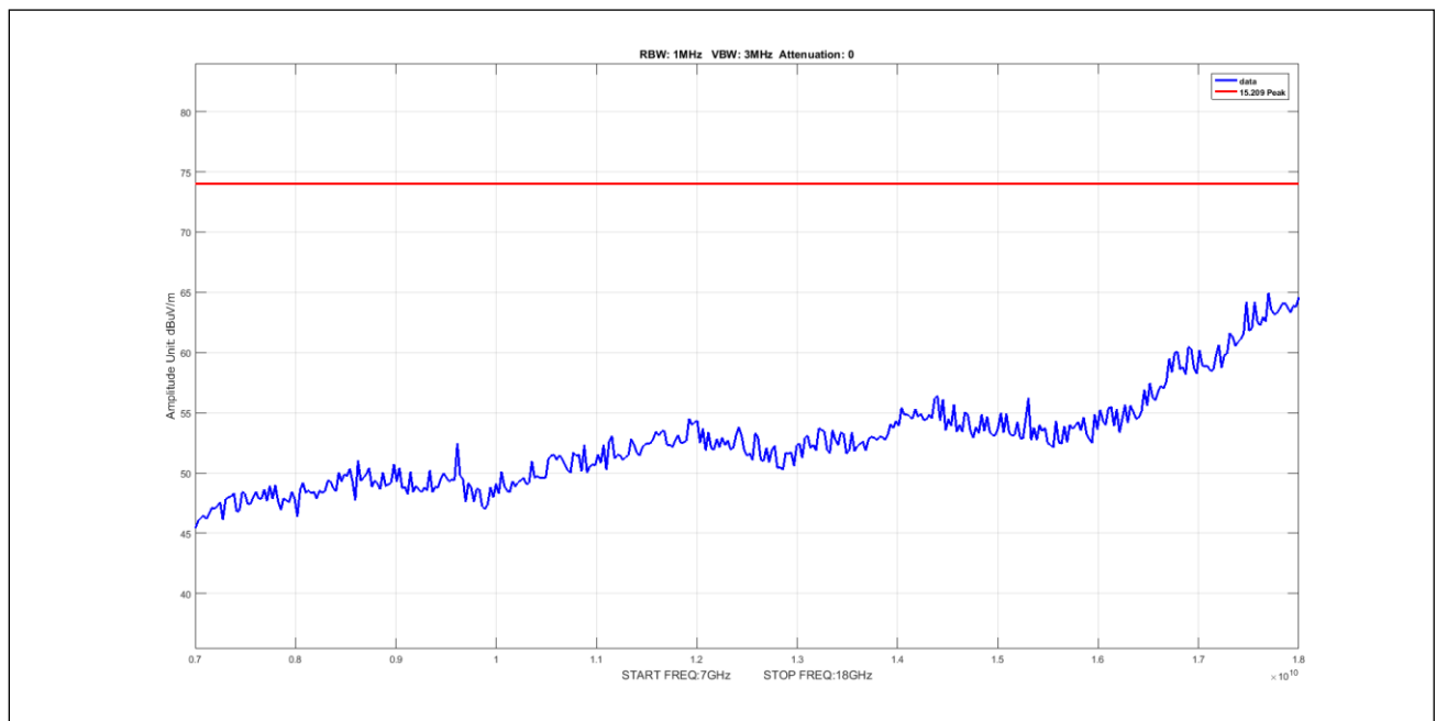
Plot 548. Undesirable Emissions, 5Omni Peak 7-18GHz 5M 5210 pow14
