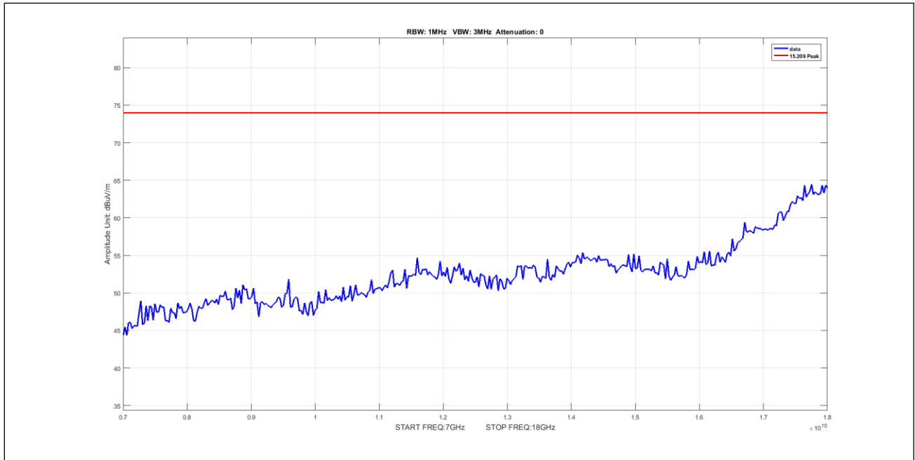
Plot 551. Undesirable Emissions, 50mni Peak 7-18GHz 10M 5210 pow17
