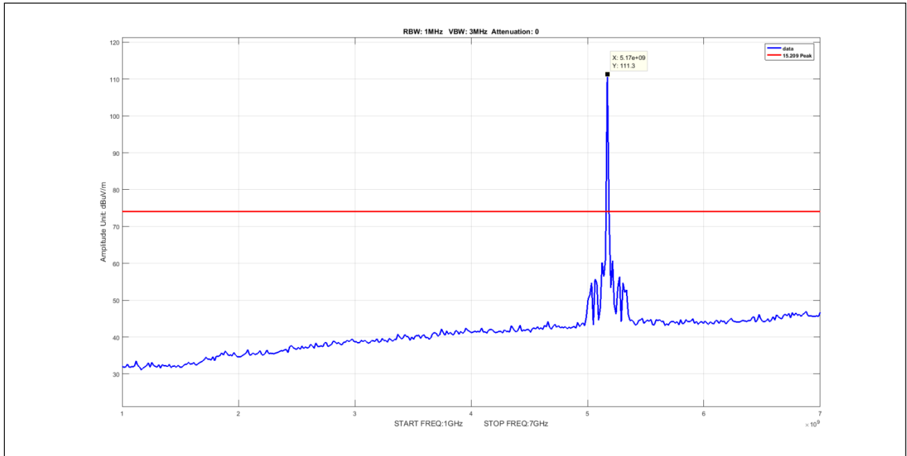
Plot 535. Undesirable Emissions, 50mni Peak 1-7GHz 5M 5170 pow14
