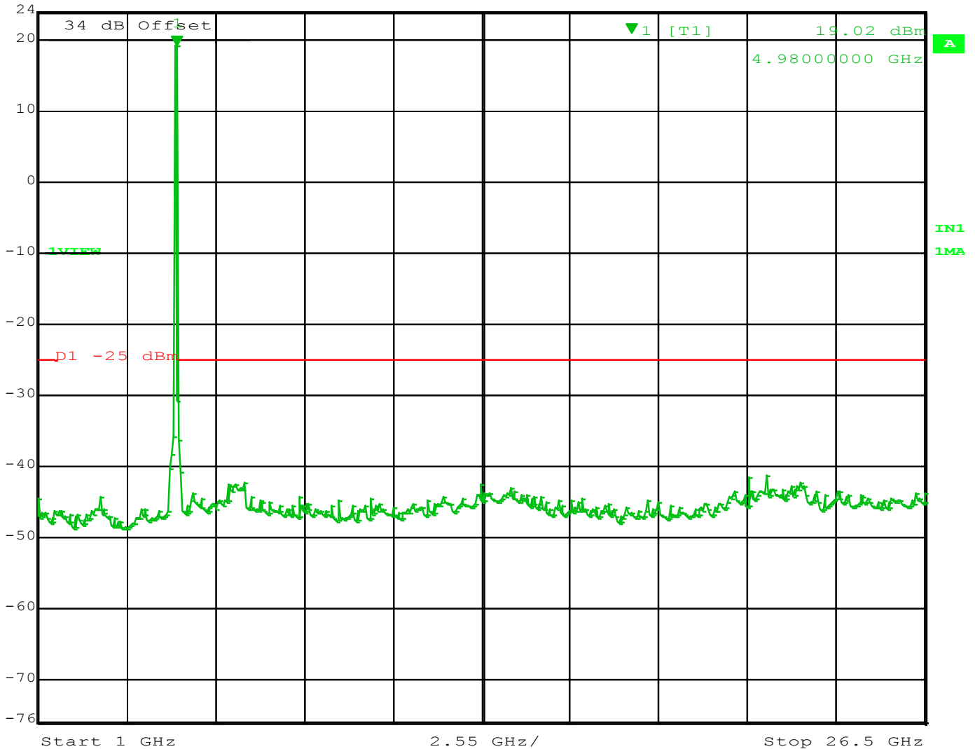
Figure 62 - Spurs 4980 MHz – 20 MHz Channel, 1 - 26.5 GHz
