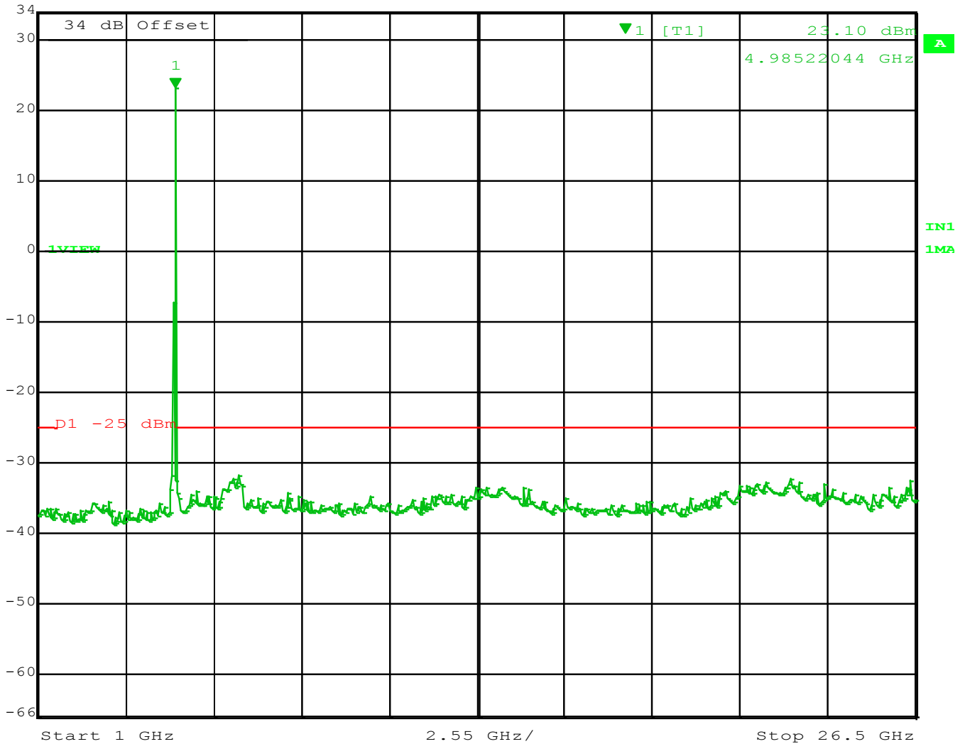
Figure 55 - Spurs 4985 MHz – 10 MHz Channel, 1 - 26.5 GHz
