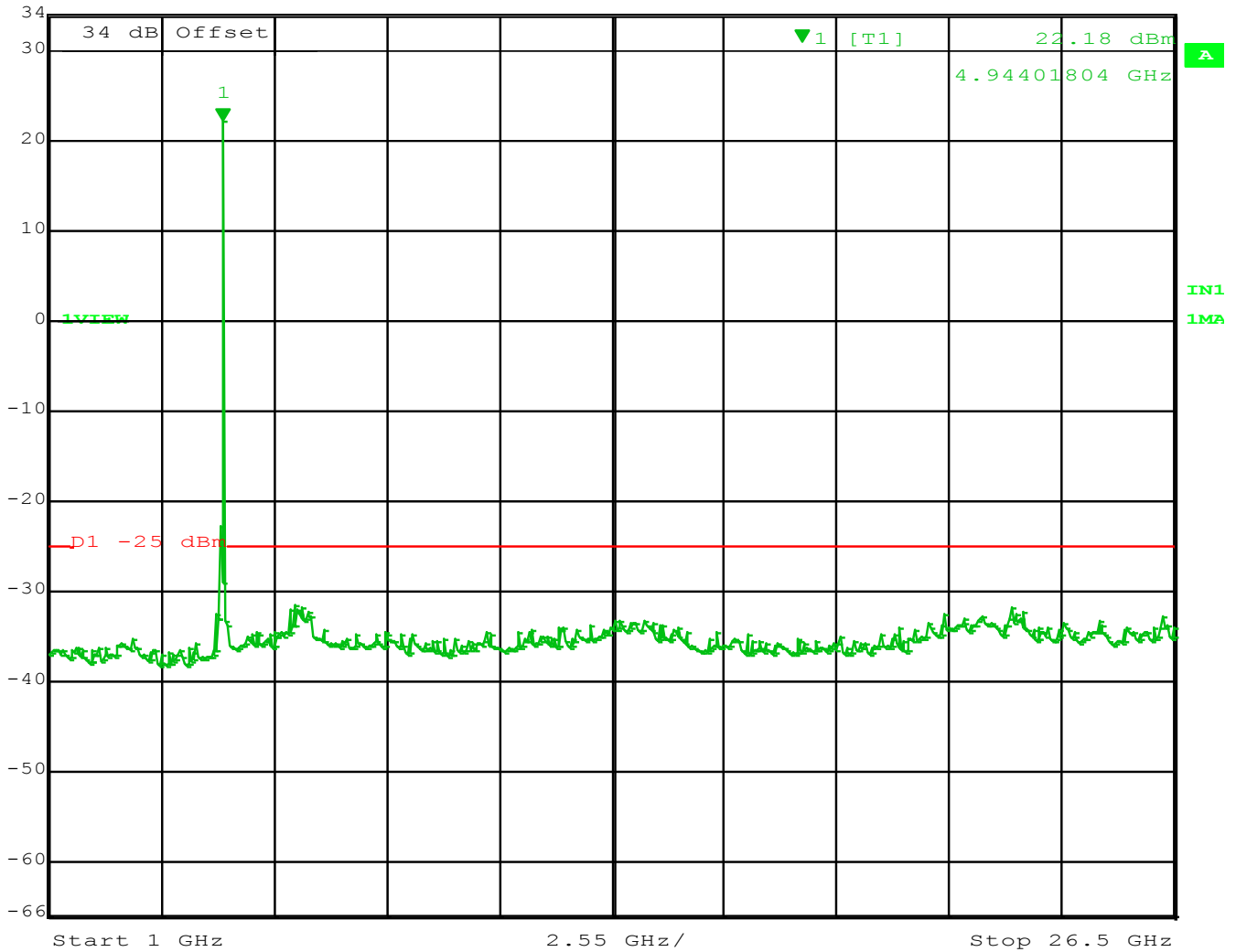
Figure 51 - Spurs 4945 MHz – 10 MHz Channel, 1 - 26.5 GHz
