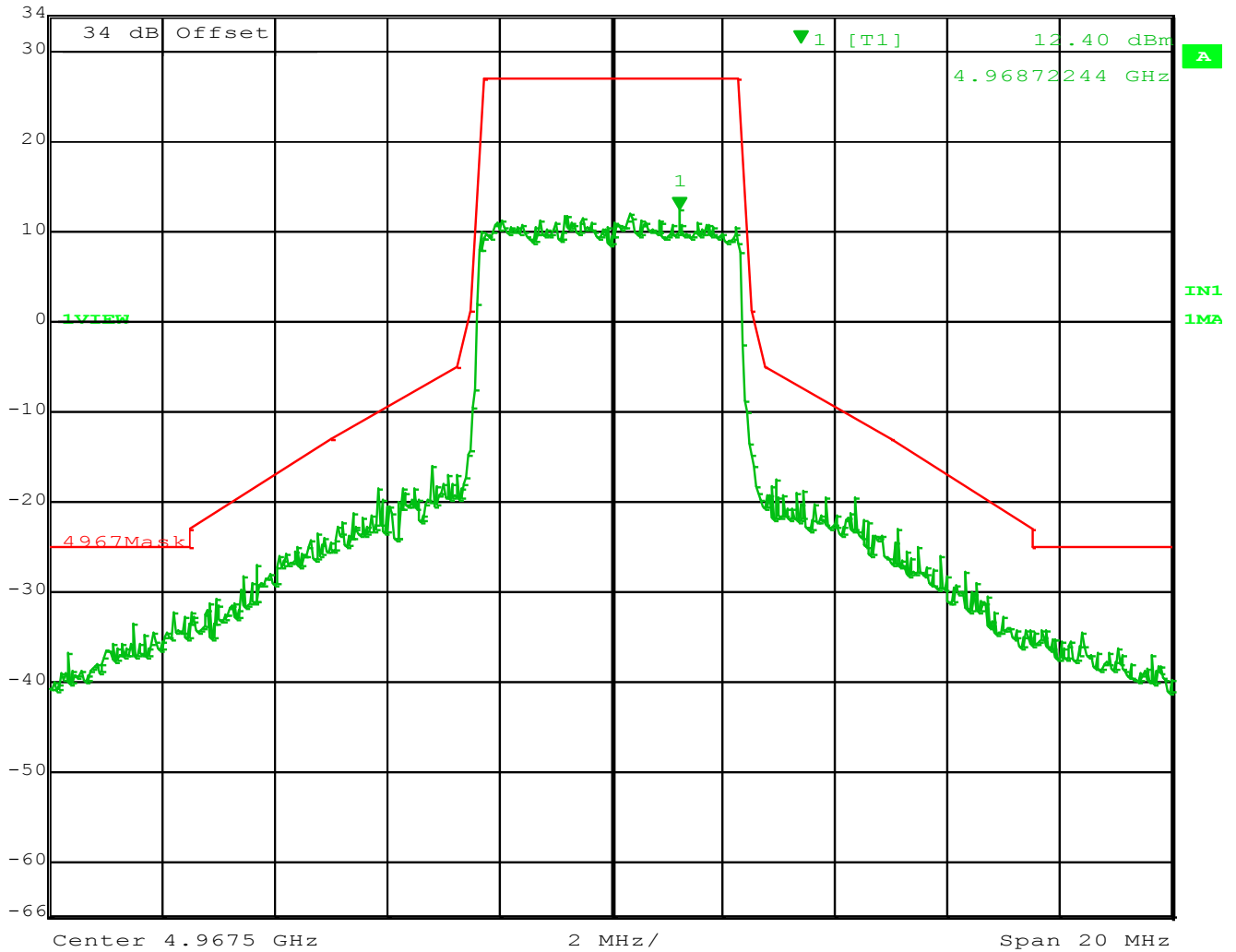
Figure 2 – Center Frequency 4967.5 MHz - 5 MHz Channel Spacing
