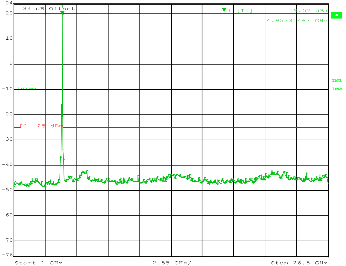
Figure 58 - Spurs 4950 MHz – 20 MHz Channel, 1 - 26.5 GHz
