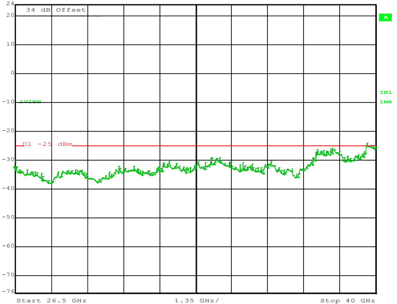
Figure 47 - Spurs 4967.5 MHz – 5 MHz Channel, 26.5 - 40 GHz
