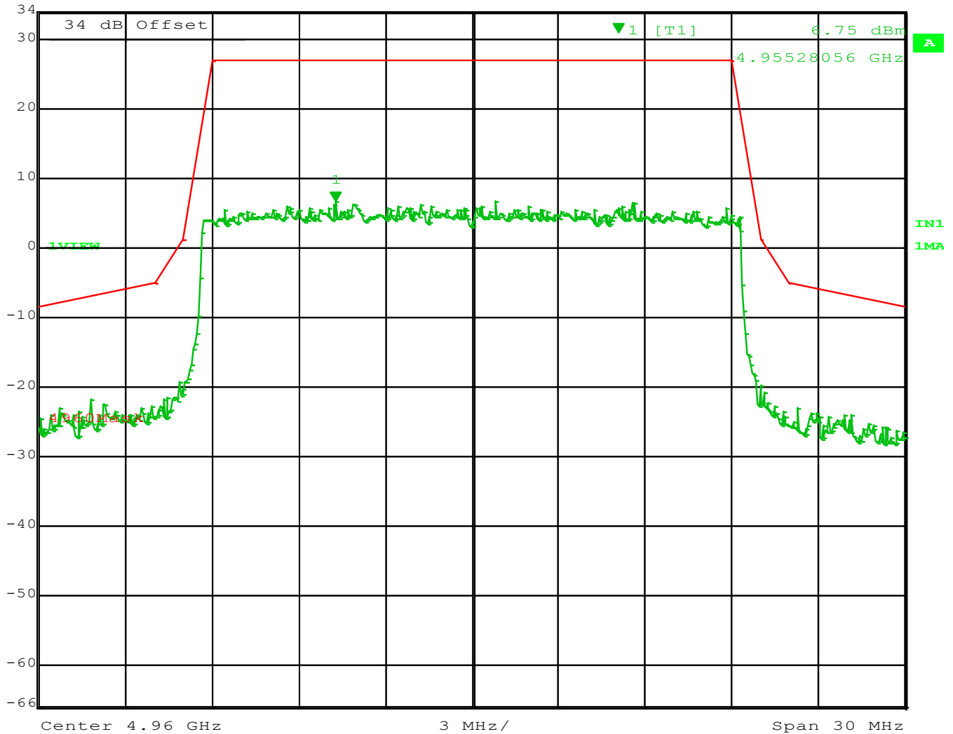
Figure 8 – Center Frequency 4960 MHz - 20 MHz Channel Spacing
