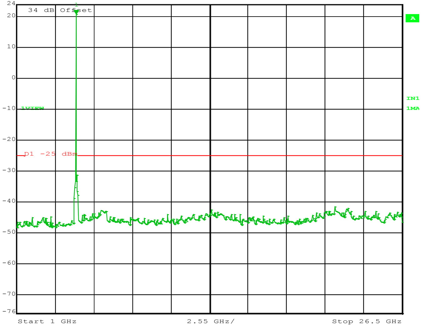
Figure 46 - Spurs 4967.5 MHz – 5 MHz Channel, 1-26.5 GHz
