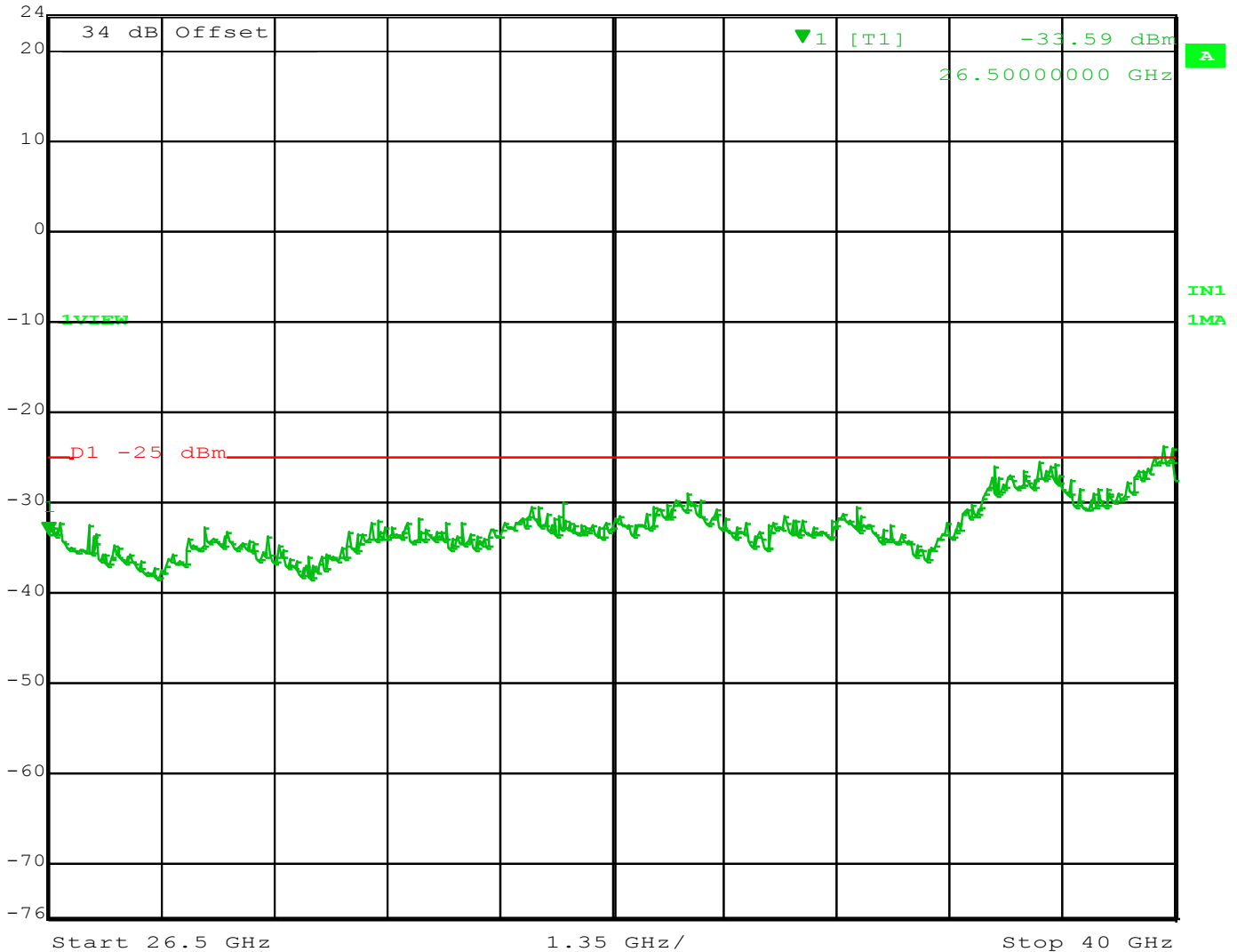
Figure 56 - Spurs 4985 MHz – 10 MHz Channel, 26.5 - 40 GHz
