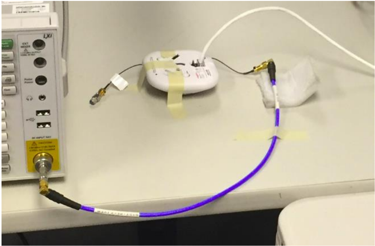
Figure 8: RF Conducted Test Setup – Close up
