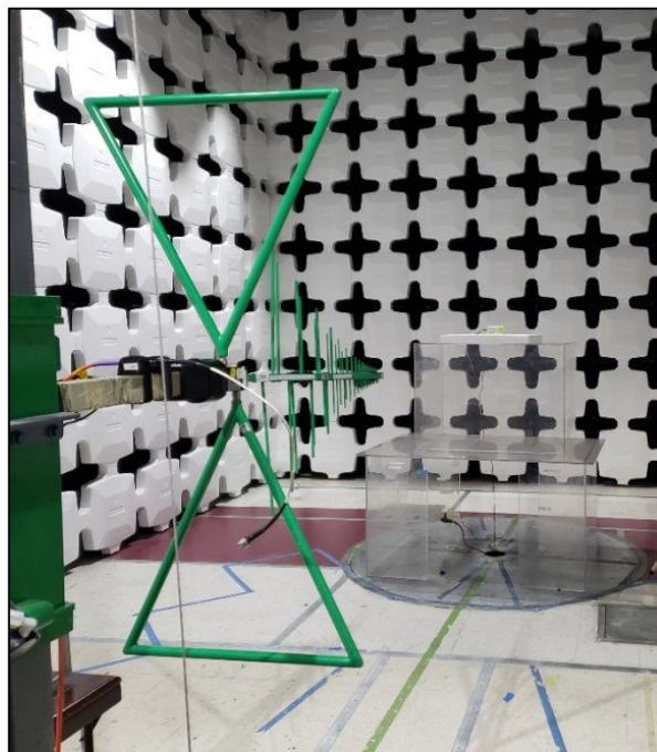
Photograph 2: Radiated Spurious Emissions Requirements, 30MHz-1GHz
