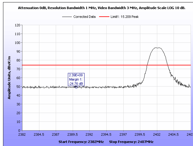
Plot 16: Radiated Band Edge, Low Channel 2402MHz, Peak
