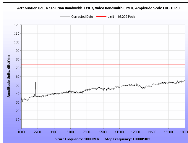
Plot 14: Radiated Spurious Emissions Requirements, High Channel 2480MHz, Peak
