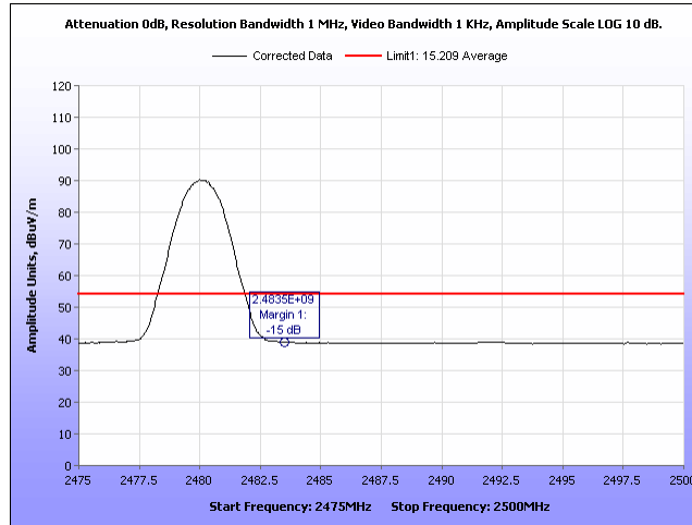
Plot 17: Radiated Band Edge, High Channel 2480MHz, Average
