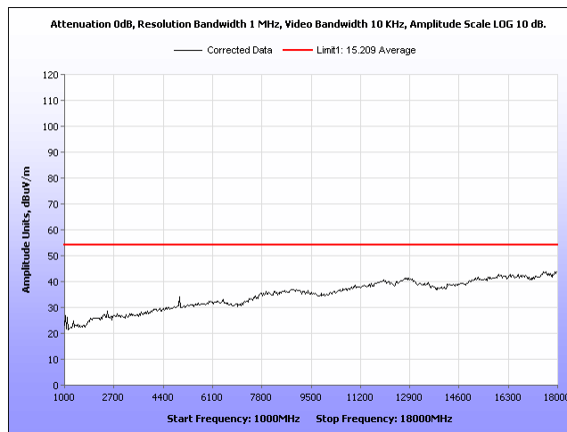
Plot 13: Radiated Spurious Emissions Requirements, High Channel 2480MHz, Average
