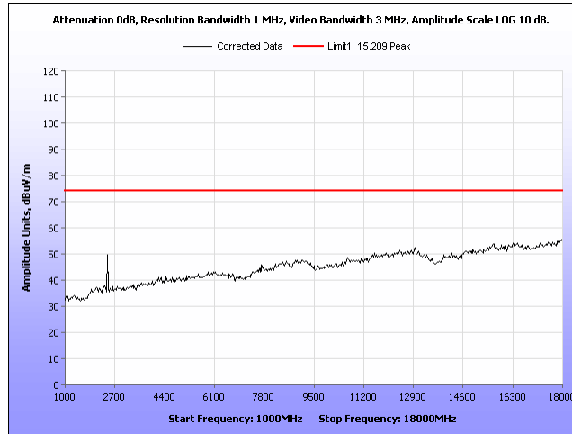
Plot 12: Radiated Spurious Emissions Requirements, Mid Channel 2442MHz, Peak
