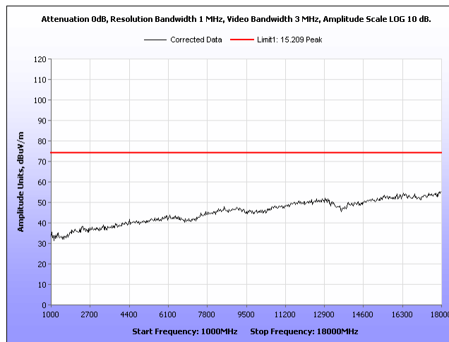
Plot 10: Radiated Spurious Emissions Requirements, Low Channel 2402MHz, Peak
