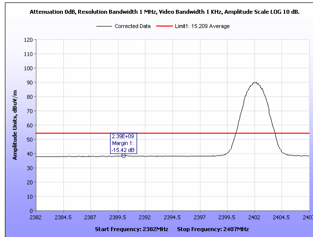
Plot 15: Radiated Band Edge, Low Channel 2402MHz, Average
