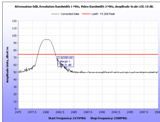
Plot 18: Radiated Band Edge, High Channel 2480MHz, Peak
