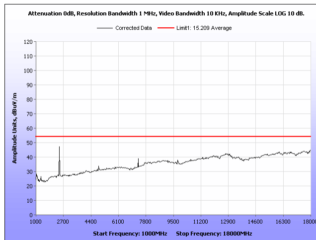
Plot 11: Radiated Spurious Emissions Requirements, Mid Channel 2442MHz, Average
