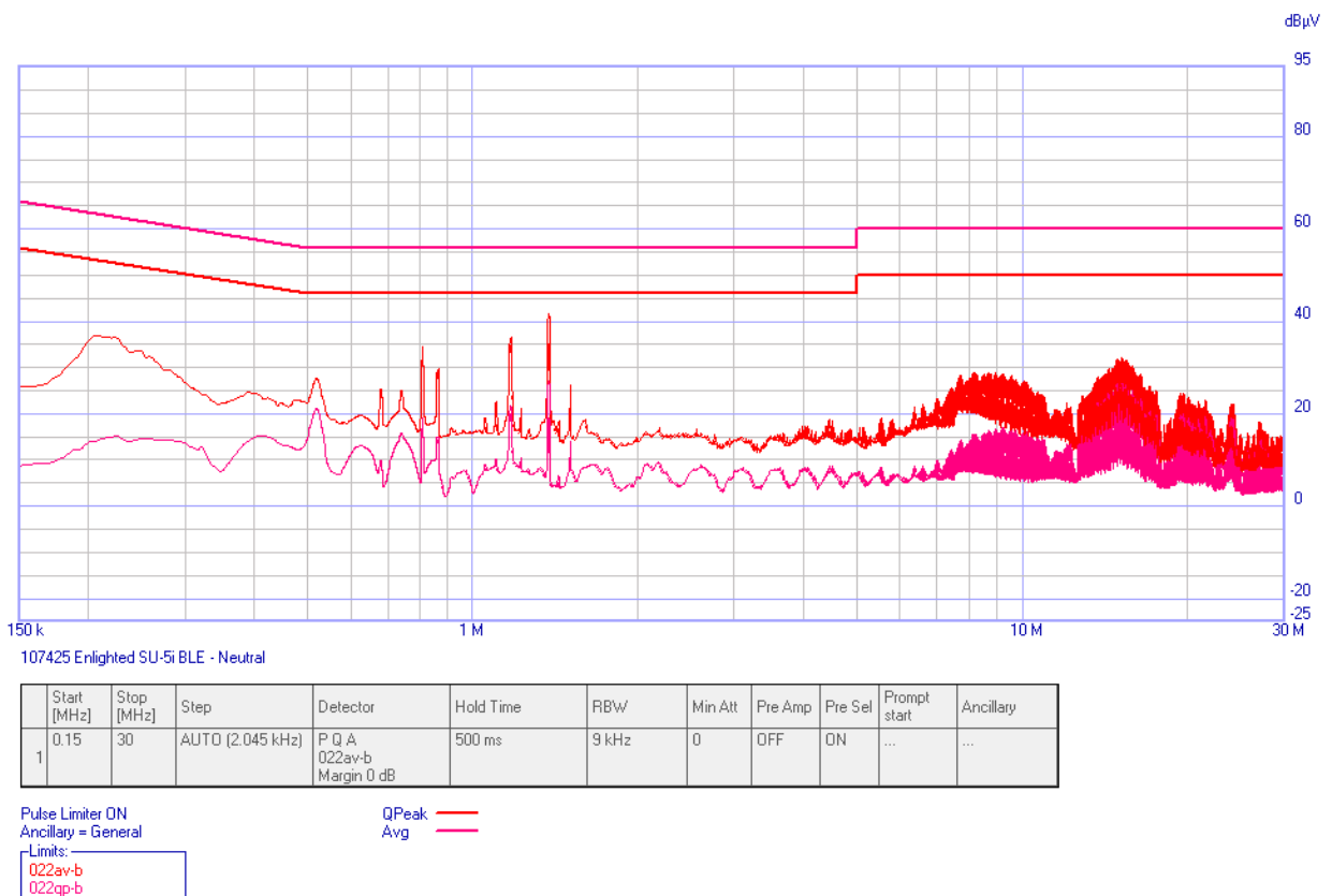
Plot 2: Conducted Emissions Limits, Neutral, Prescan
