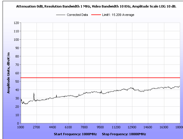
Plot 9: Radiated Spurious Emissions Requirements, Low Channel 2402MHz, Average
