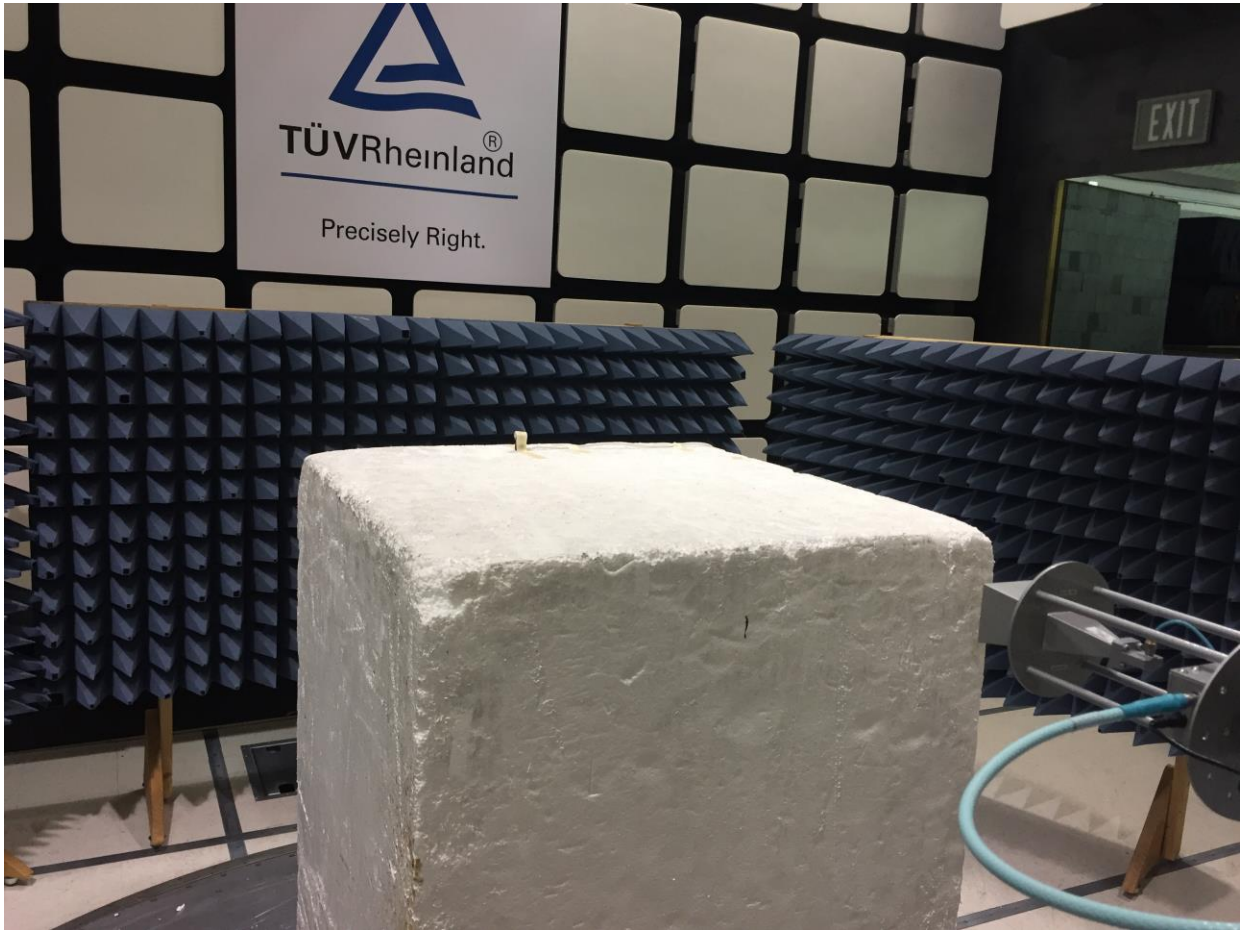
Figure 5: Test Setup for 18 GHz to 25GHz(Front View)
