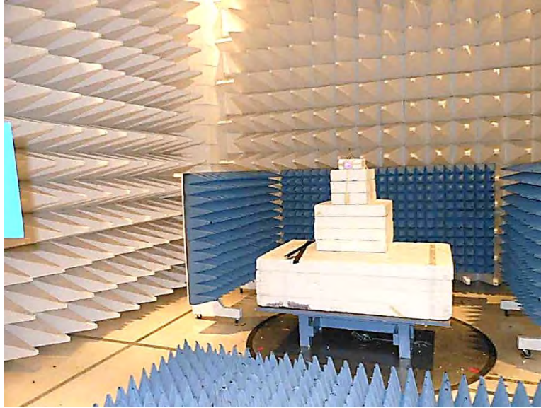
Configuration 2, 12 – 25GHz
