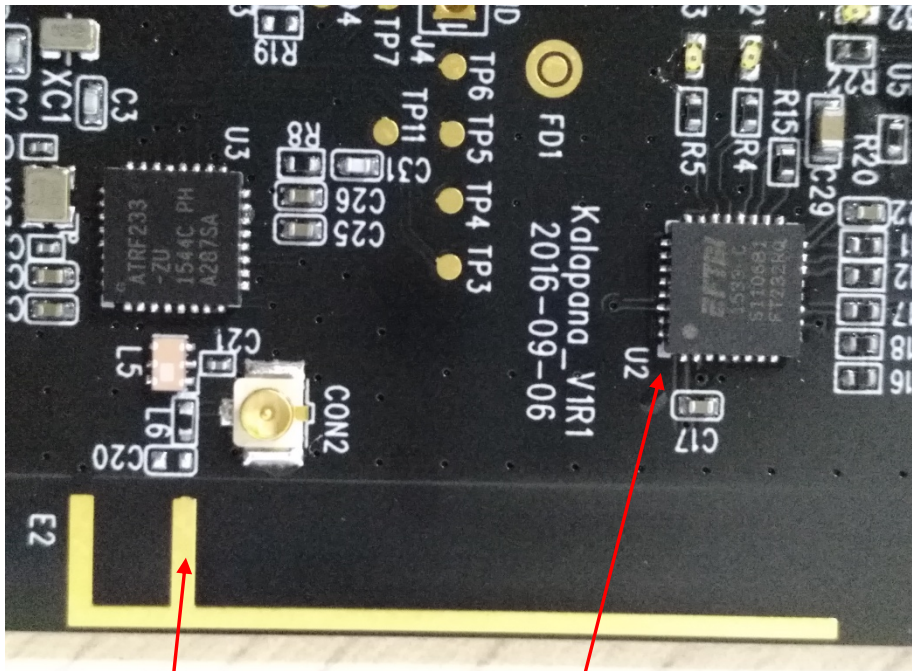
802.15.4 ANTENNA
