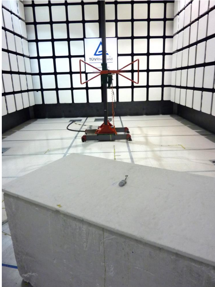
Figure 2: Test Setup for 30MHz to 1GHz (Rear View – EUT Horizontal)
