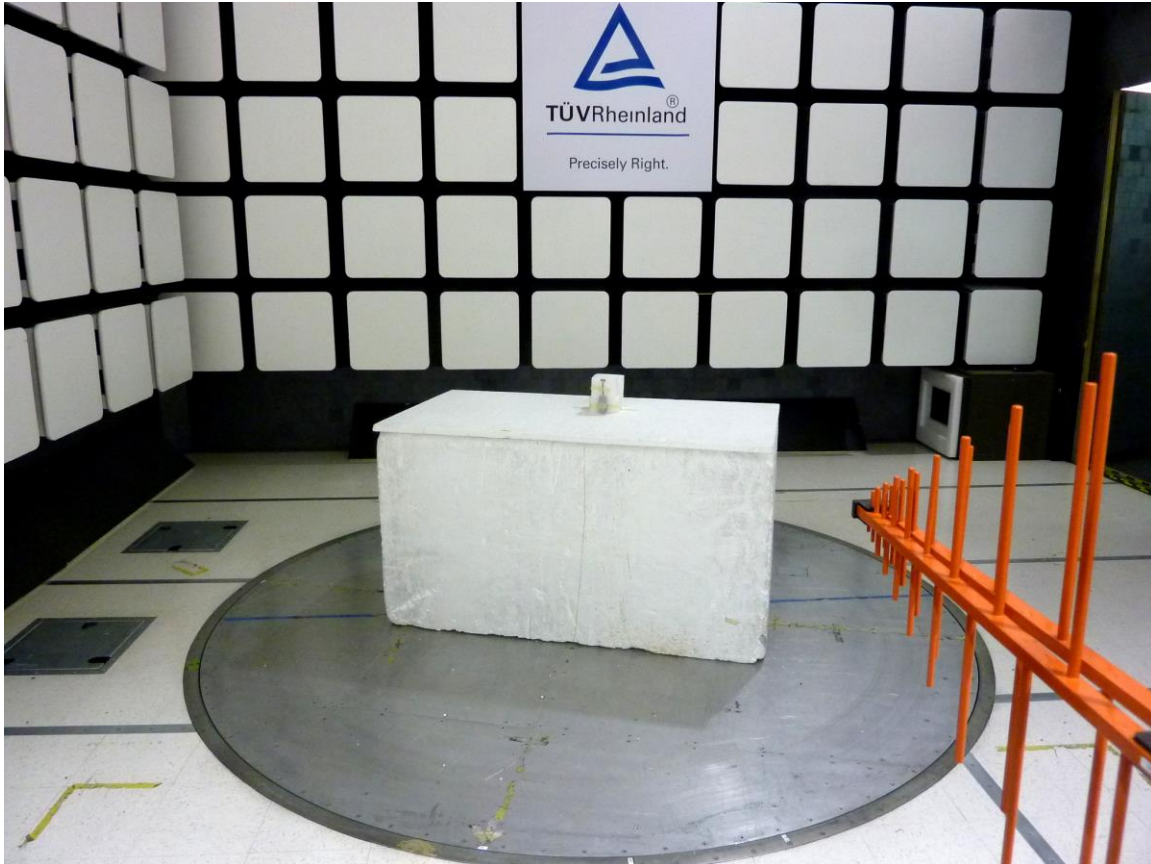
Figure 1: Test Setup for 30MHz to 1GHz (Front View – EUT vertical)
