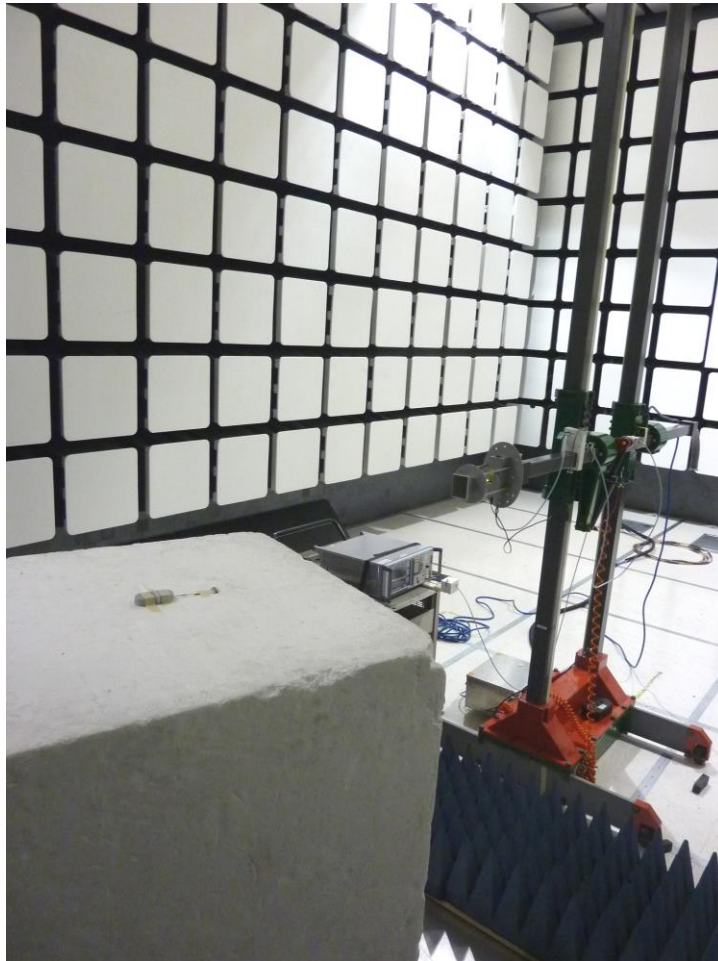
Figure 6: Test Setup for 18GHz to 26GHz another View
