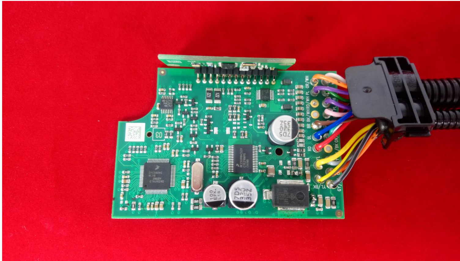
Figure 3: Topside with UHF module lifted to show topside components
