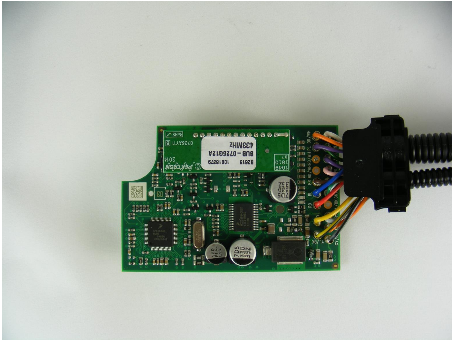
Figure 2: KCU2 Internal, Topside
