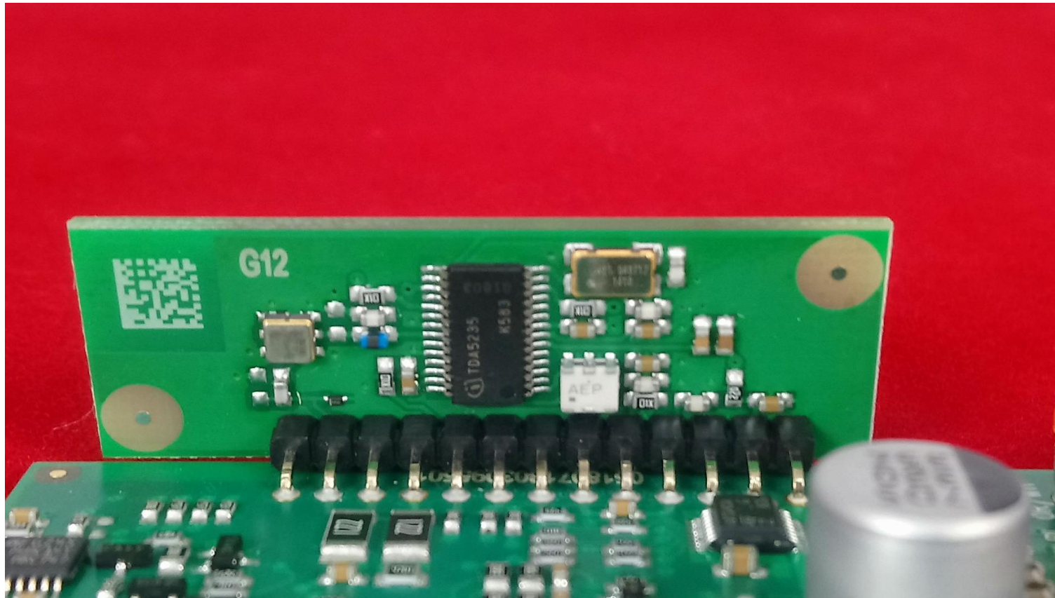
Figure 4: Topside with UHF module lifted to show UHF underside components
