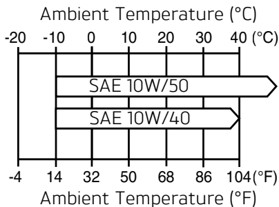
Oil Viscosity Temperature Range
