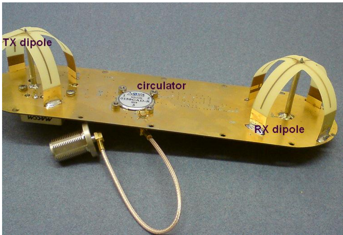
Main Board assembly.
