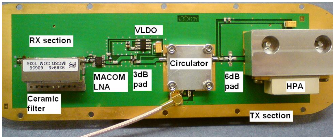
Main board.
