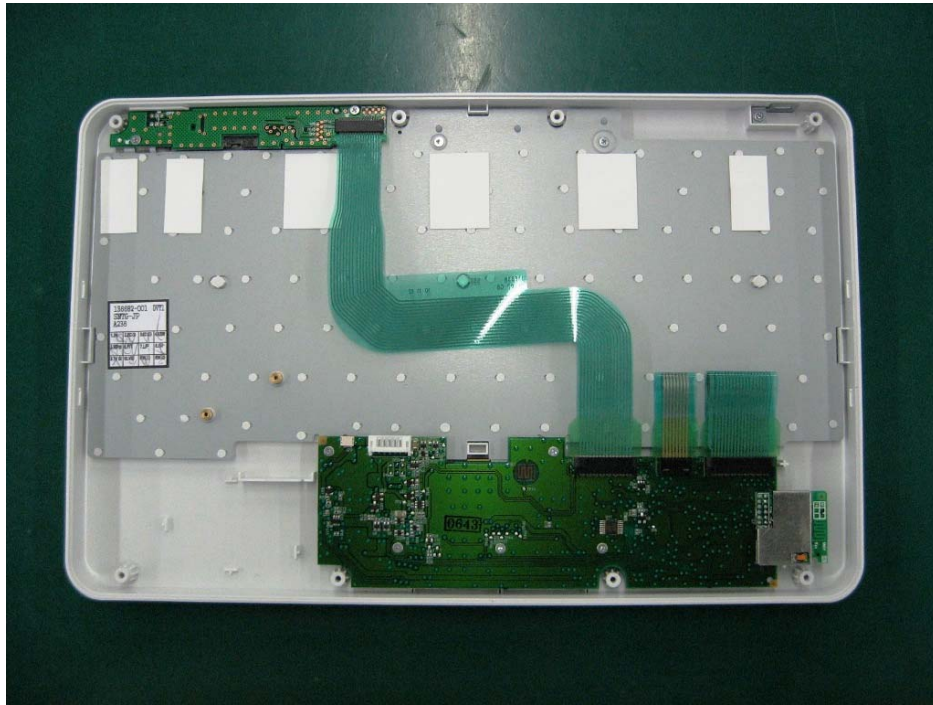
Internal Top View installed board
