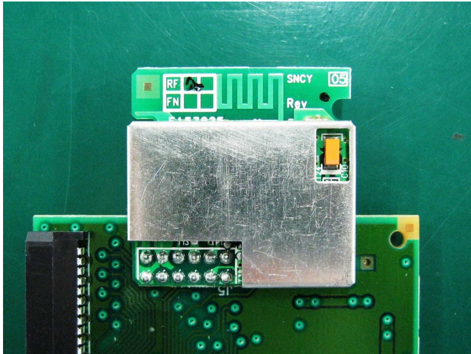
Front View (RF module with shield)
