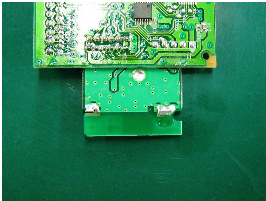
Rear View (RF module)
