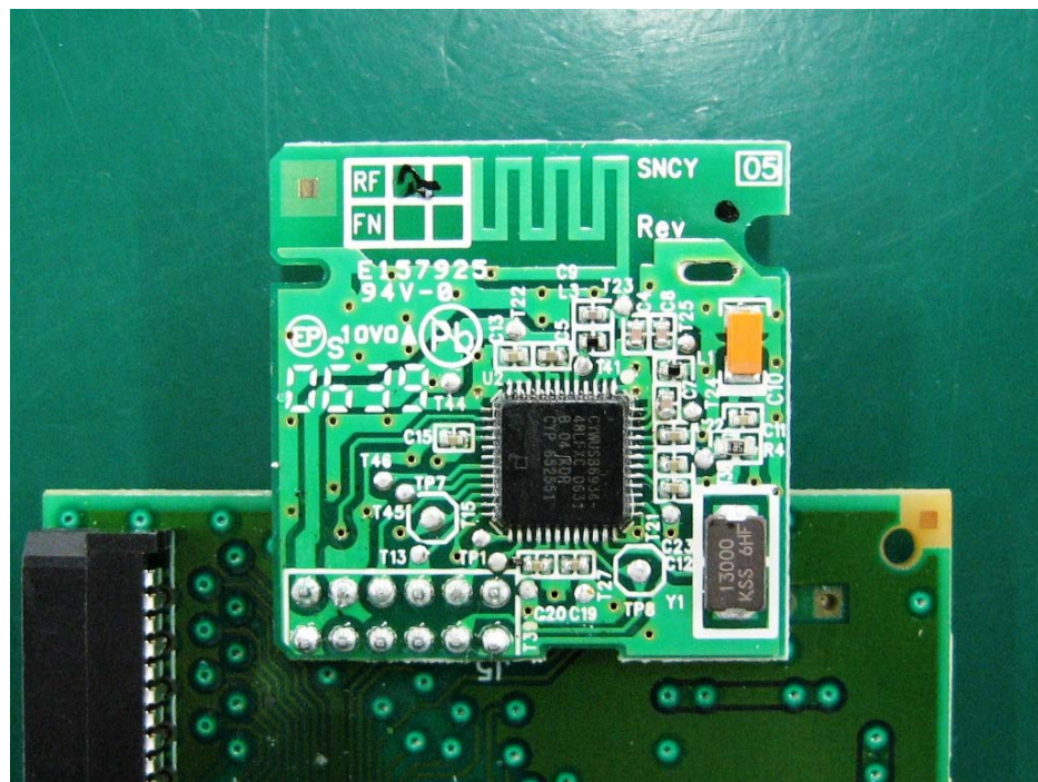
Front View (RF module without shield)
