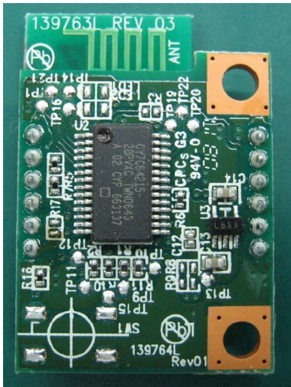
Receiver (VGP-WRC4) Top view
