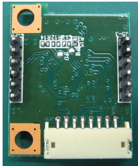
Main PCBA Bottom view
