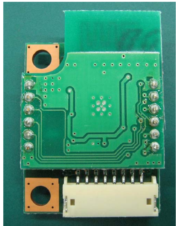
Receiver Bottom view
