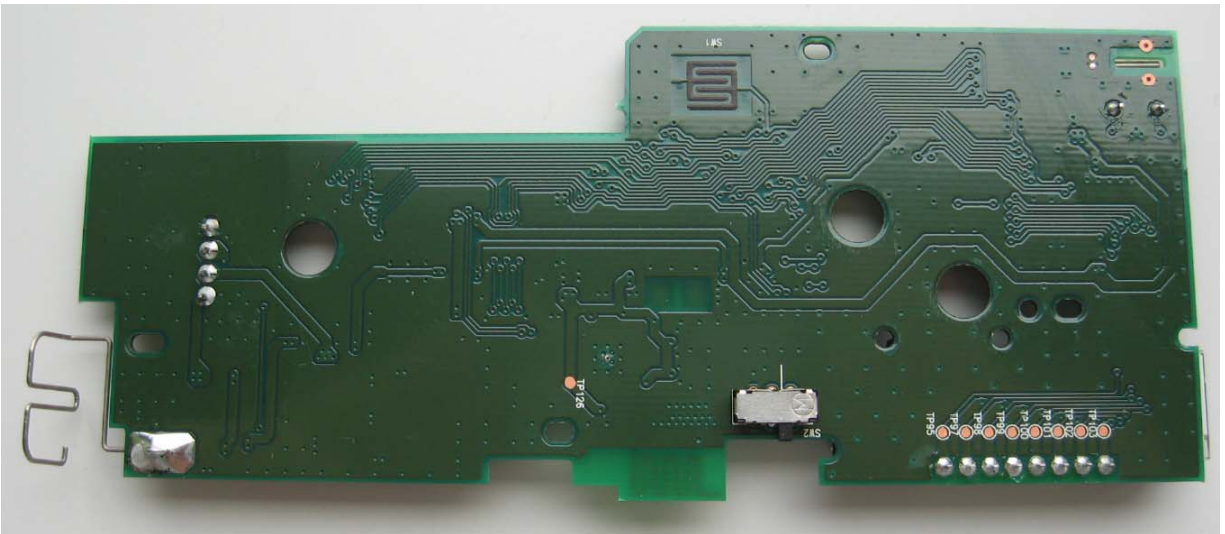
PCBA Bottom of view
