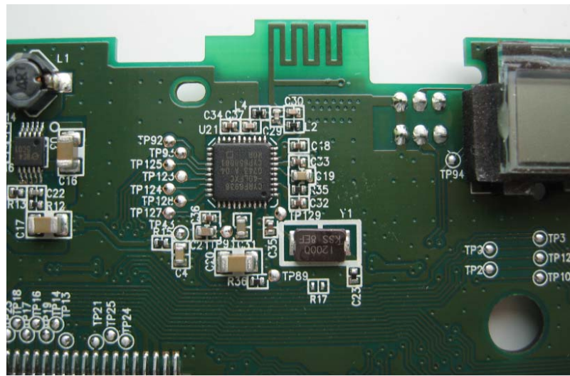
Detail of RF part
