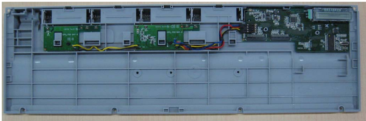
Open Keyboard Bottom side of Inside Keyboard
