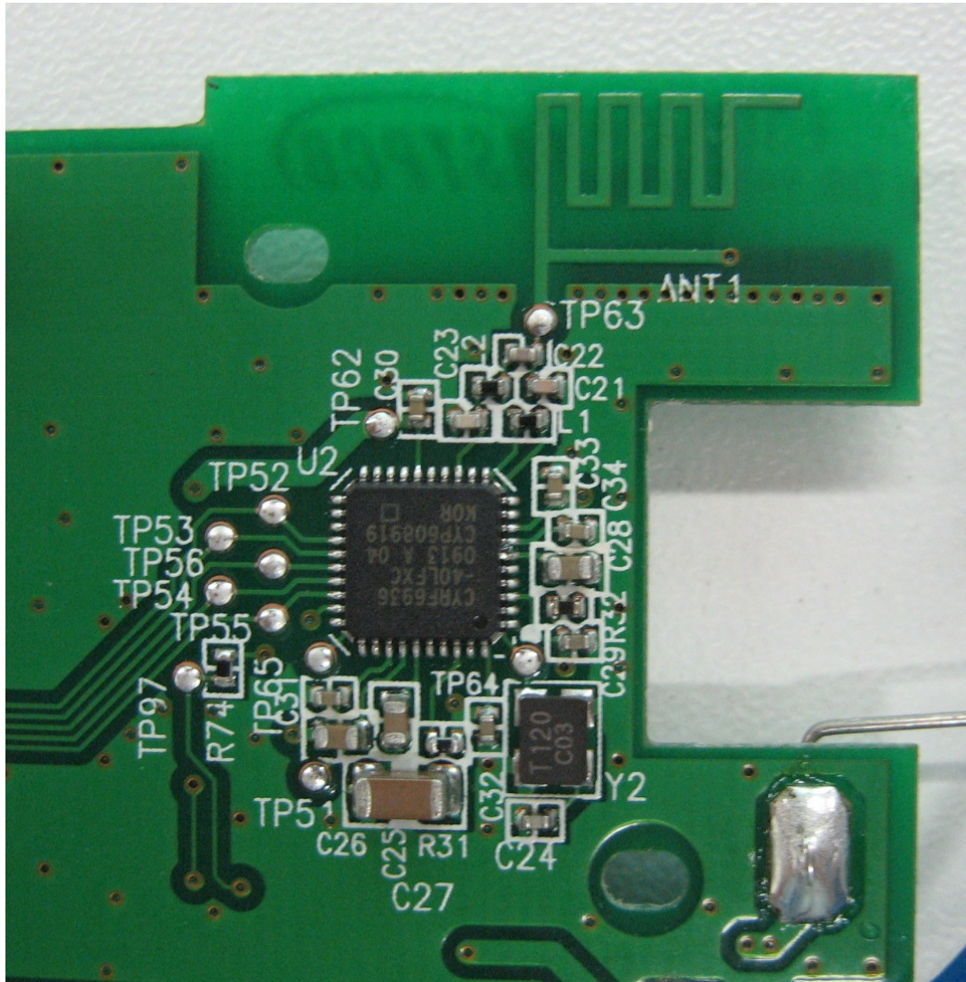
Detail of RF part on PCBA
