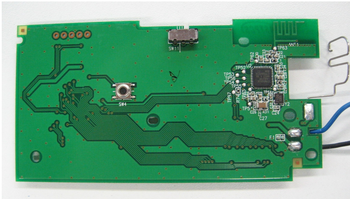
PCBA Bottom of view
