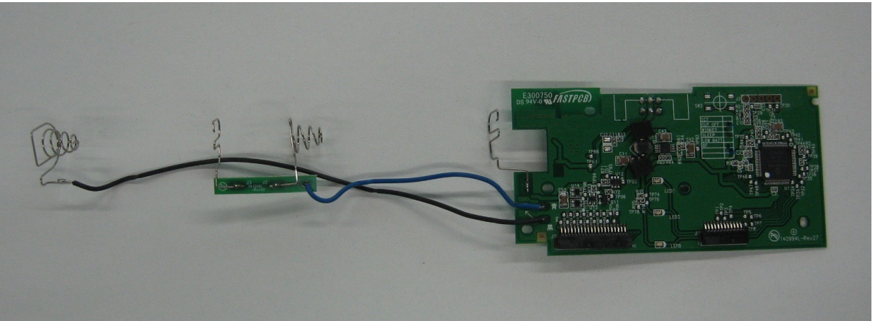
PCBA view
