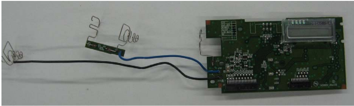
PCBA view
