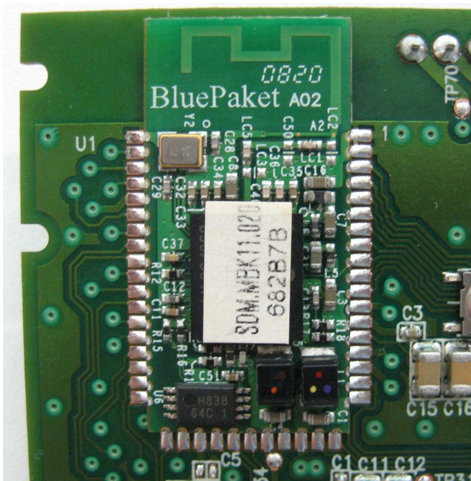
PCBA Bottom of view
