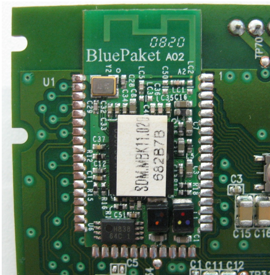
Detail of RF part on PCBA
