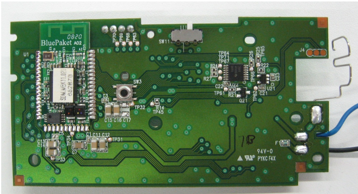
PCBA Bottom of view
