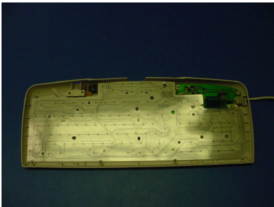
12.8 MEMBRANE CONTACTS
