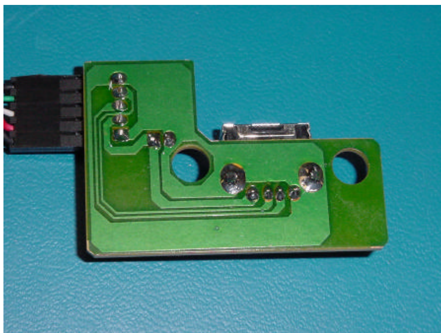
12.4 SOLDER SIDE USB PORT
