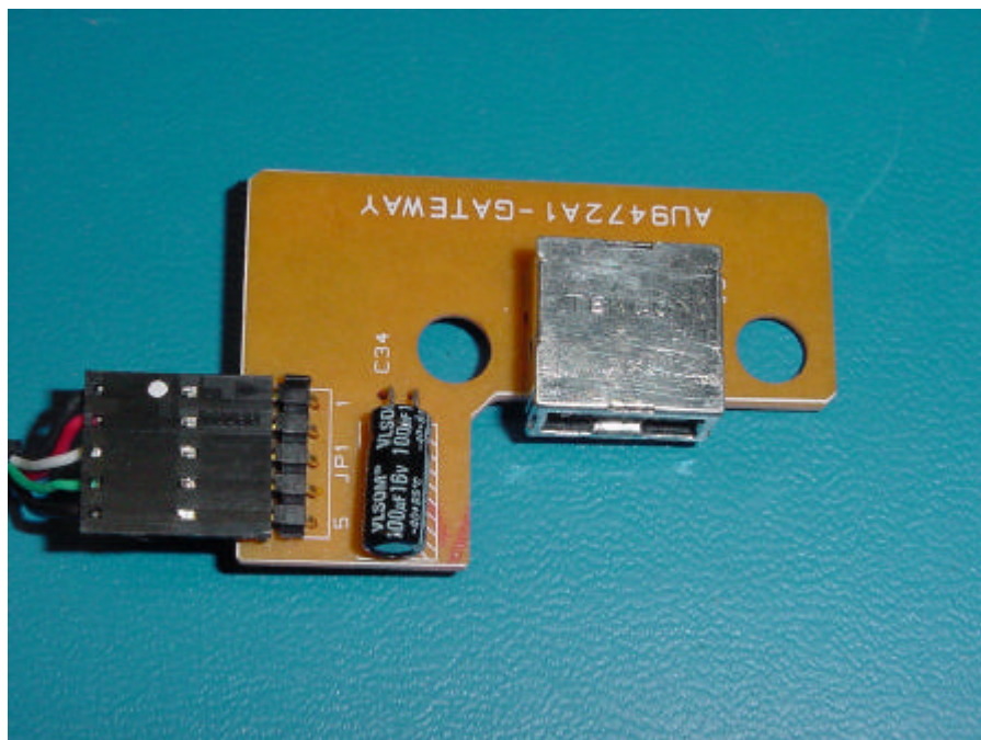
12.3 COMPONENT SIDE USB PORT
