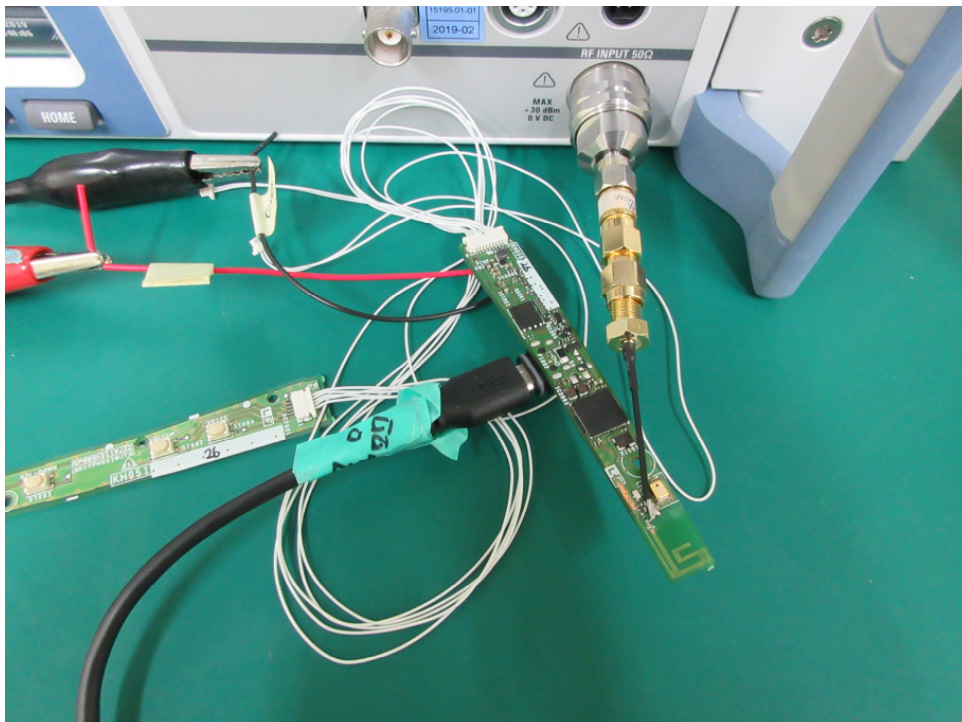
Photograph 8: Set-up Conducted testing (View 2)
