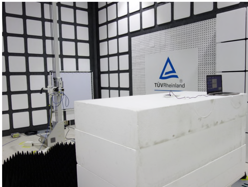
Photograph 6: Set-up for Spurious Emissions (Back View 2)
