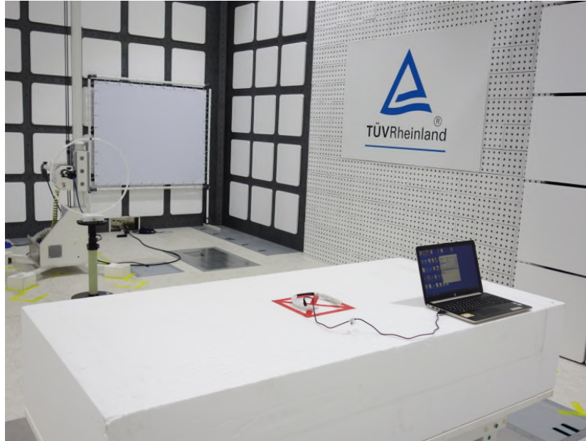
Photograph 5: Set-up for Spurious Emissions (Back View 2)
