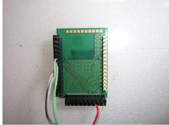
Rear View (Reference)
