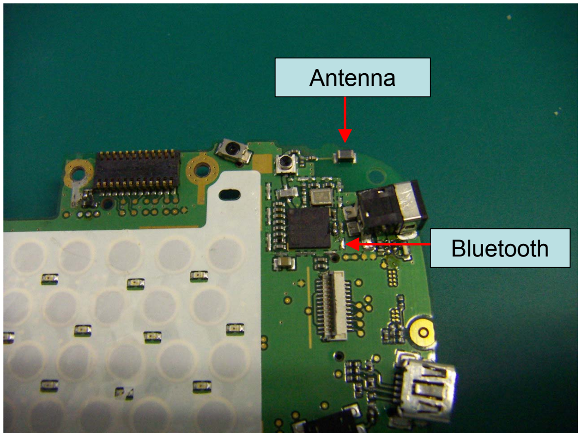
Photo of Bluetooth Module
