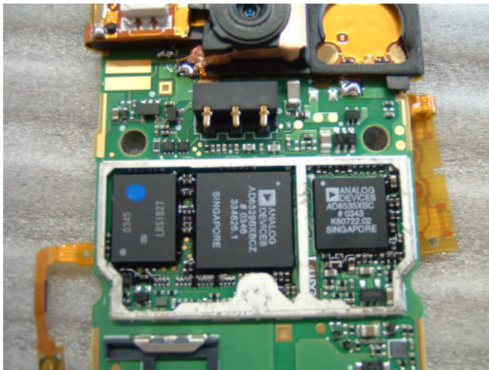
Middle Layer Side B Detail
