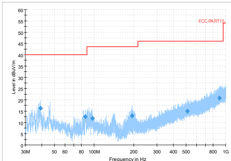
Frequency Range: 30MHz-1GHz Detector: QP mode Modulation type: 8DPSK
