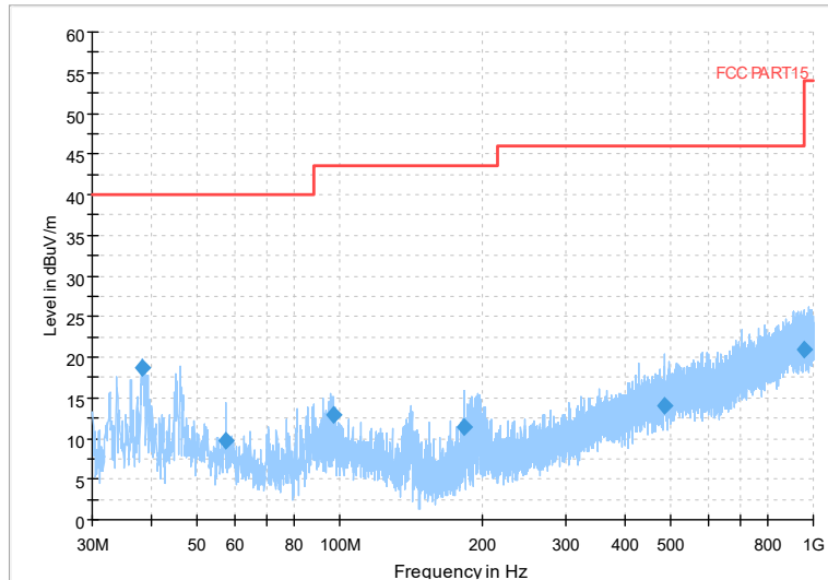
Frequency Range: 30MHz -1GHz Detector:QP mode Modulation type: 802.11n(HT20)
