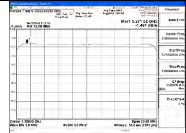
Mode:802.11be EHT20 Tone:242T Frequency:5280MHz Ant:Chain0
