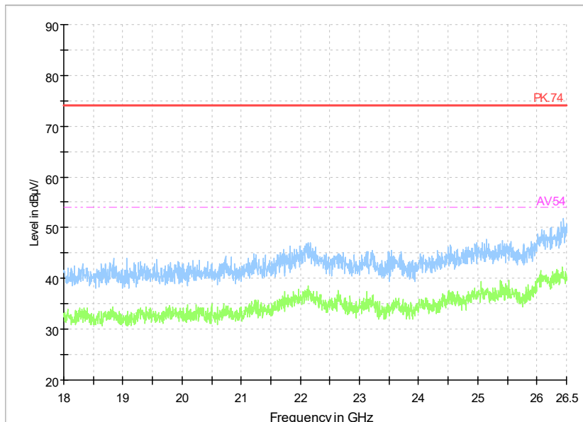
Pic8. Radiated emission (18GHz – 26GHz)
