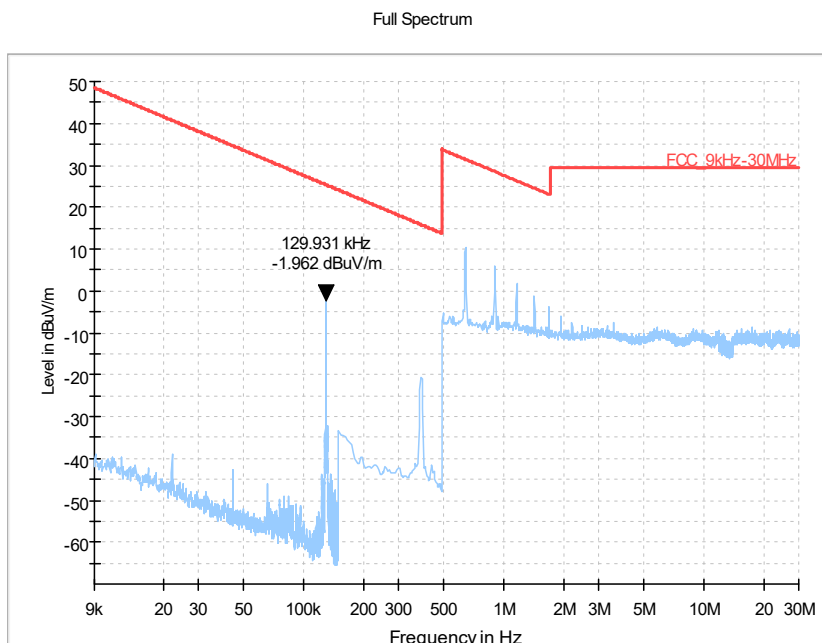
Pic4. Radiated emission(9KHz – 30MHz)
