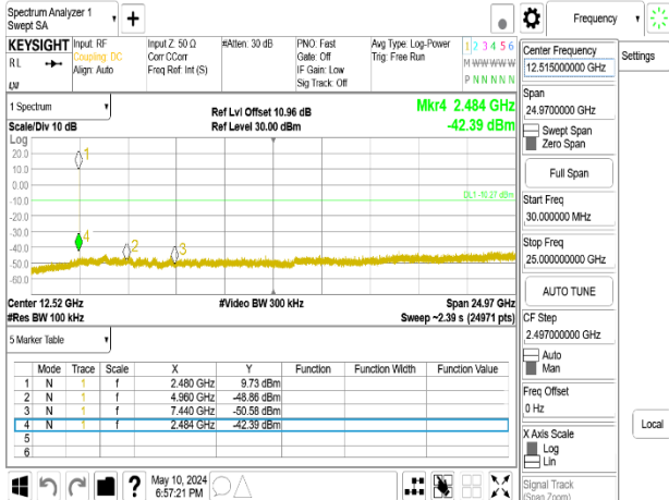
Spurious Emission_8DPSK_3M_DH5_2480MHz_Chain0
