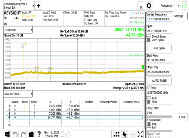
Spurious Emission_pi/4DQPSK_2M_DH5_2402MHz_Chain1
