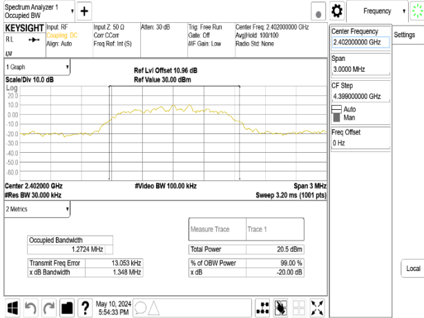
OBW 20dB_π/4DQPSK_2M_DH5_2402MHz_Chain1
