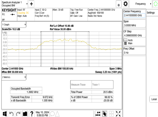
OBW 20dB_π/4DQPSK_2M_DH5_2441MHz_Chain0
