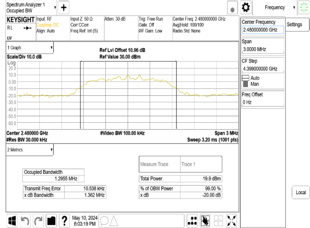
OBW 20dB_π/4DQPSK_2M_DH5_2480MHz_Chain1
