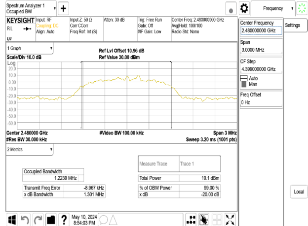
OBW 20dB_8DPSK_3M_DH5_2480MHz_Chain1
