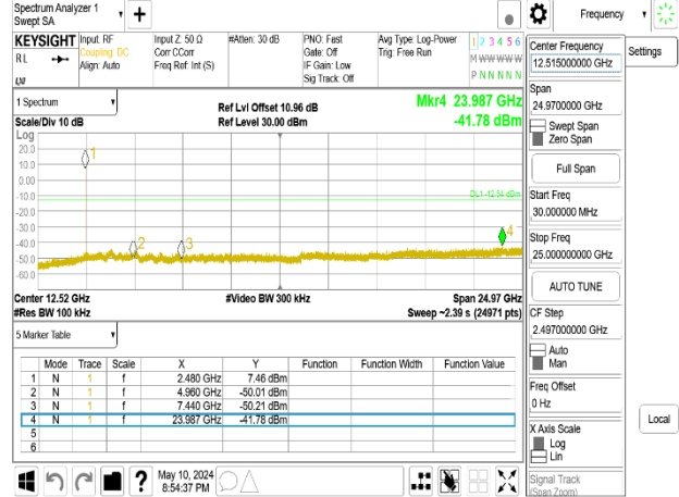
Spurious Emission_8DPSK_3M_DH5_2480MHz_Chain1
