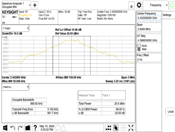
OBW 20dB_GFSK_1M_DH5_2402MHz_Chain1
