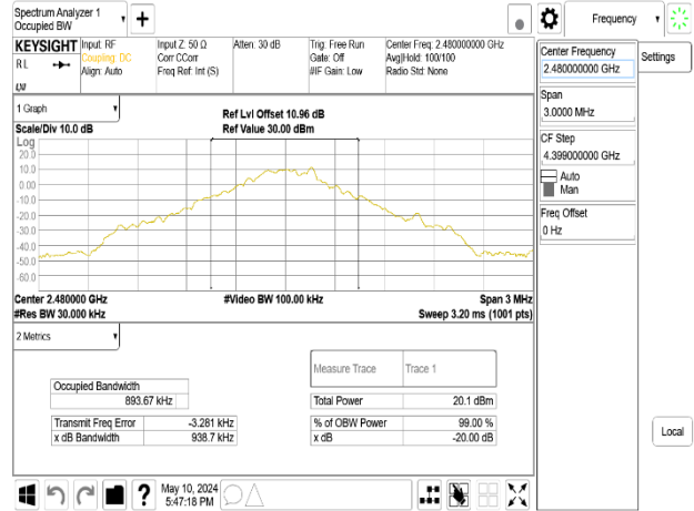
OBW 20dB_GFSK_1M_DH5_2480MHz_Chain1
