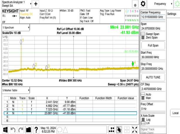
Spurious Emission_8DPSK_3M_DH5_2441MHz_Chain1
