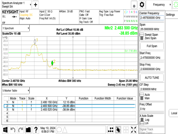
Band Edge_8DPSK_3M_DH5_2480MHz_Chain1
