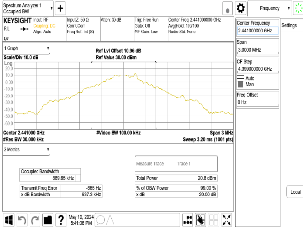
OBW 20dB_GFSK_1M_DH5_2441MHz_Chain0
