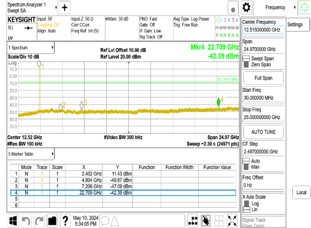
Spurious Emission_GFSK_1M_DH5_2402MHz_Chain1
