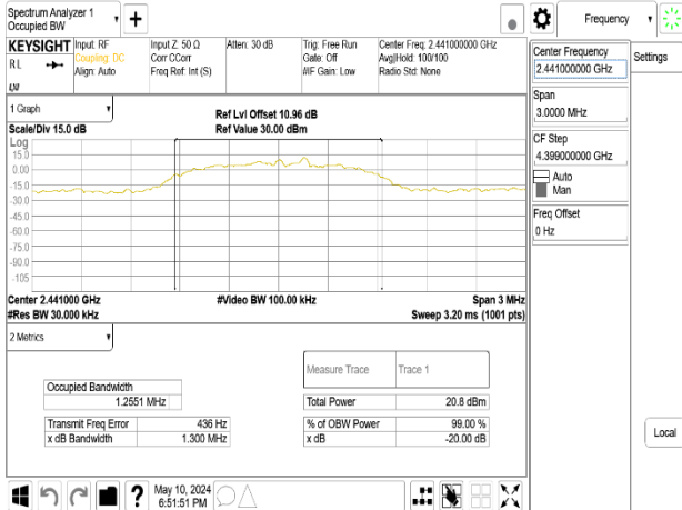
OBW 20dB_8DPSK_3M_DH5_2441MHz_Chain0
