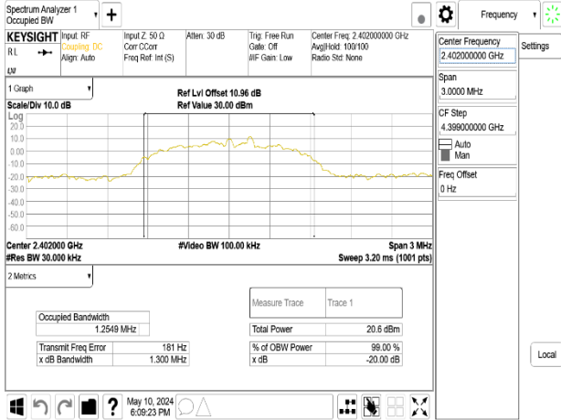
OBW 20dB_8DPSK_3M_DH5_2402MHz_Chain1
