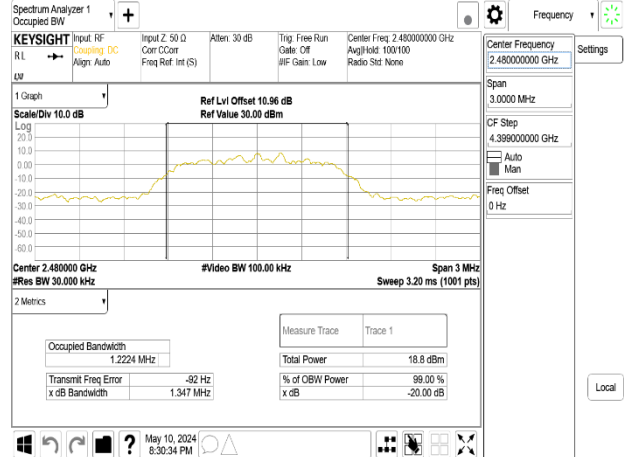
OBW 20dB_π/4DQPSK_2M_DH5_2480MHz_Chain1
