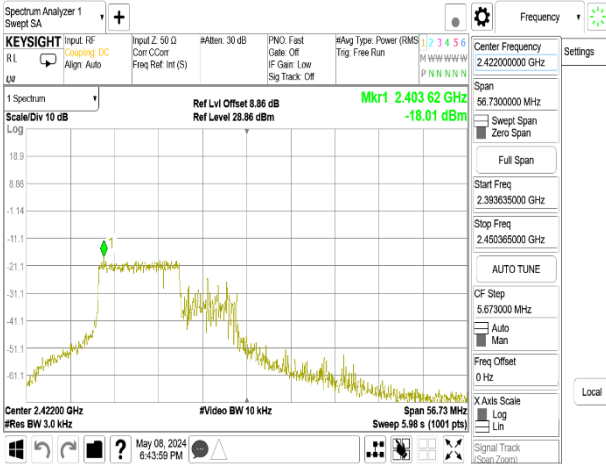
802.11be_40MHz_Chain1_2422MHz_52+26_MRU1
