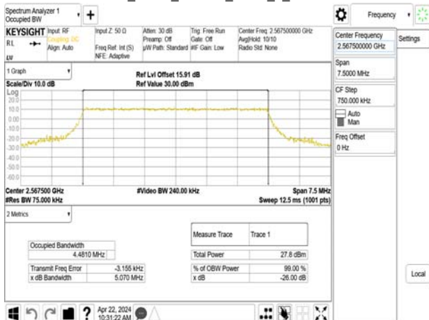
Band7_5MHz_64QAM_RB25_0_CH21425
