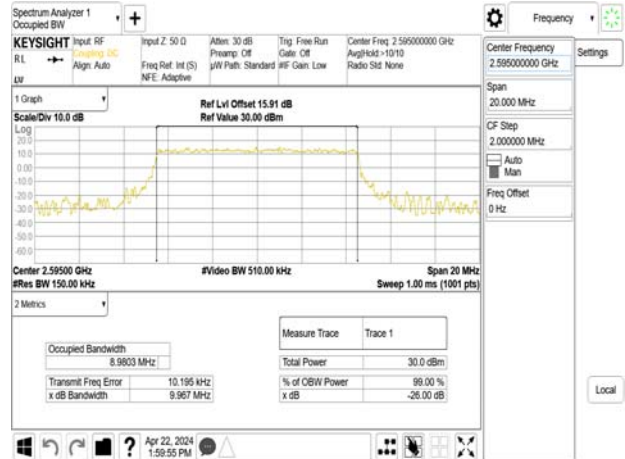
Band38_10MHz_QPSK_RB50_0_CH38200
