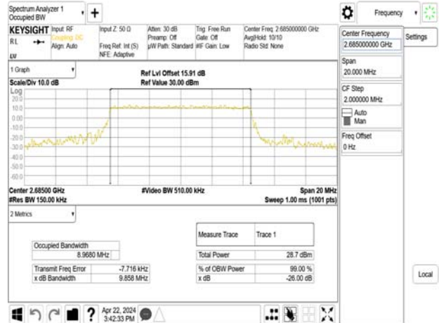
Band41_10MHz_64QAM_RB50_0_CH41540
