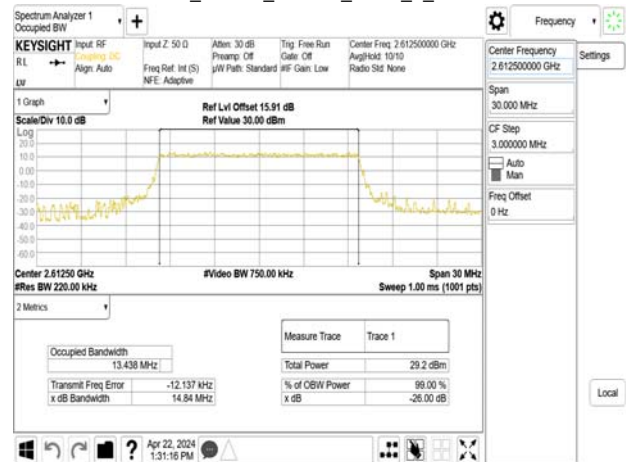
Band38_15MHz_16QAM_RB75_0_CH38175
