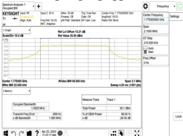
Band66_1.4MHz_QPSK_RB6_0_CH132665
