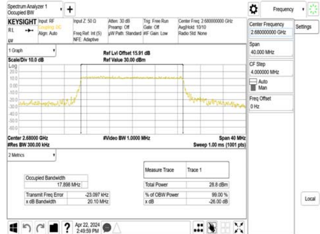
Band41_20MHz_64QAM_RB100_0_CH41490
