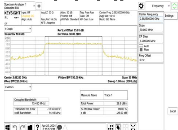
Band41_15MHz_16QAM_RB75_0_CH41515
