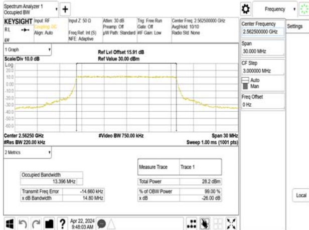
Band7_15MHz_64QAM_RB75_0_CH21375
