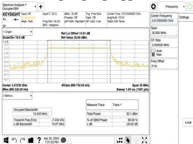
Band38_15MHz_QPSK_RB75_0_CH38175
