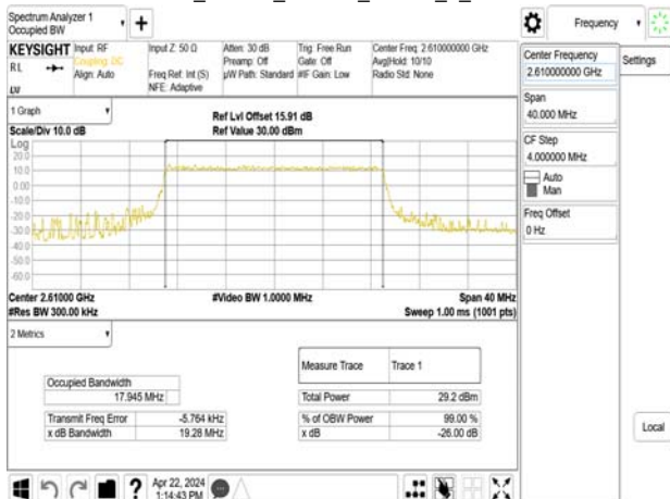
Band38_20MHz_16QAM_RB100_0_CH38150
