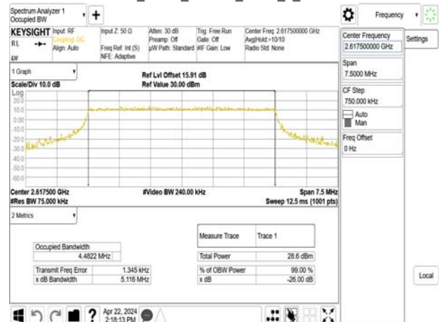
Band38_5MHz_16QAM_RB25_0_CH38225
