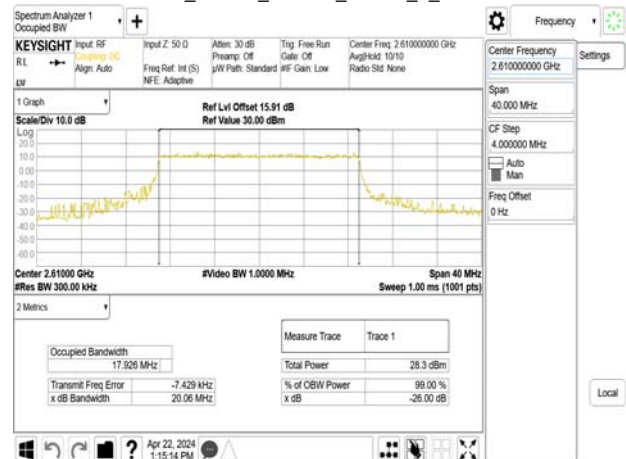
Band38_20MHz_64QAM_RB100_0_CH38150
