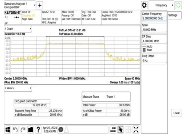
Band38_20MHz_QPSK_RB100_0_CH38000
