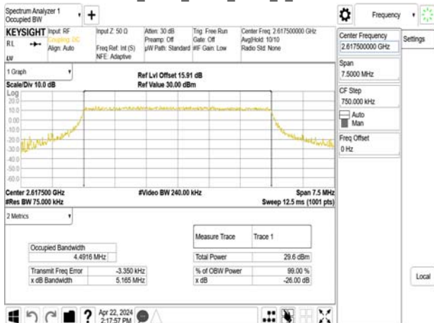
Band38_5MHz_QPSK_RB25_0_CH38225
