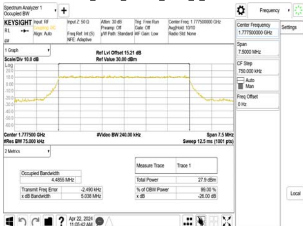
Band66_5MHz_64QAM_RB25_0_CH132647
