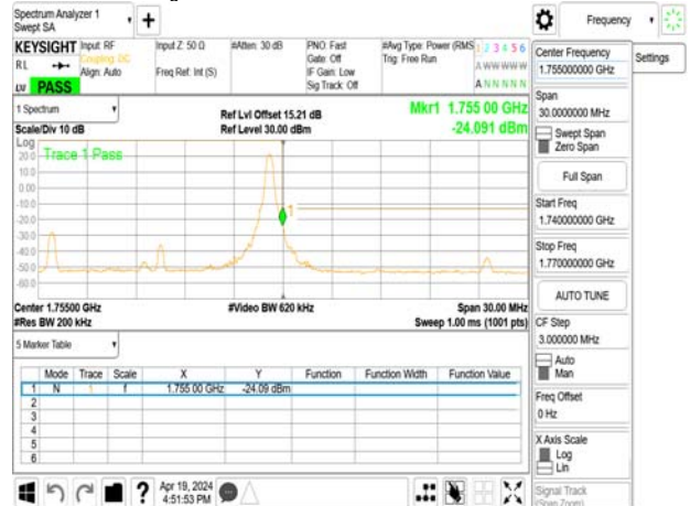
Band Edge_Band4_15MHz_OPSK_RB1_74_CH20325
