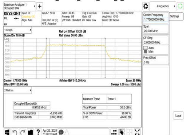
Band66_10MHz_QPSK_RB50_0_CH132622
