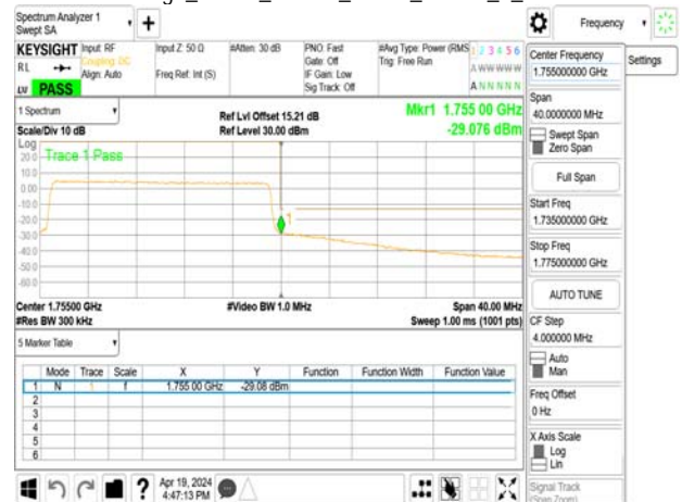
Band Edge_Band4_20MHz_OPSK_RB100_0_CH20300
