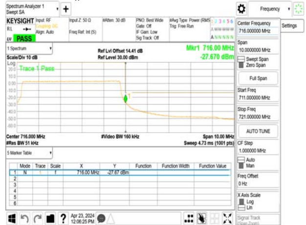
Band Edge_Band12_10MHz_OPSK_RB1_0_CH23060
