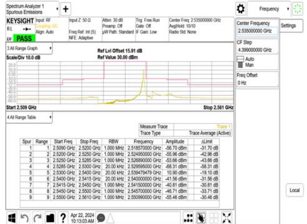
Emission Mask_Band7_10MHz_OPSK_RB1_49_CH21100
