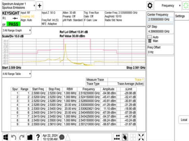
Emission Mask_Band7_10MHz_OPSK_RB1_0_CH21100
