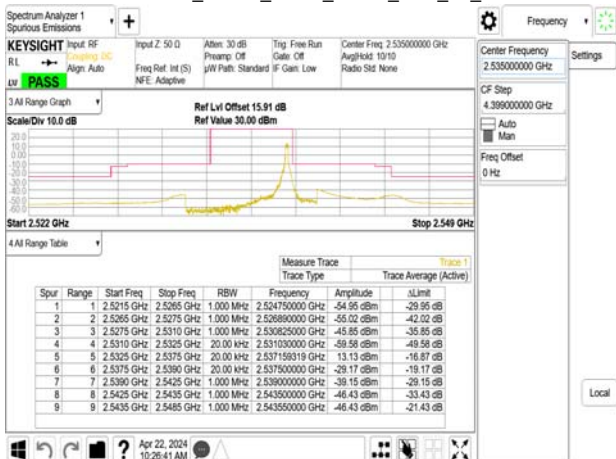
Emission Mask_Band7_5MHz_QPSK_RB1_24_CH21100
