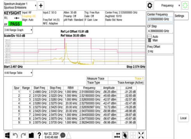
Emission Mask_Band7_15MHz_QPSK_RB1_0_CH21100
