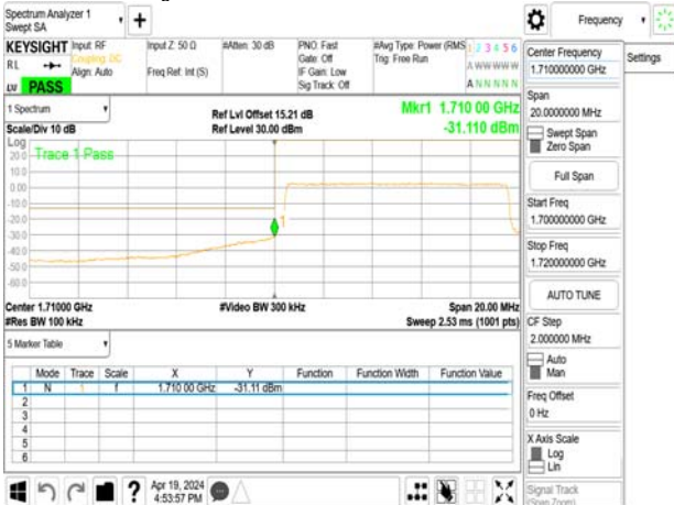
Band Edge_Band4_10MHz_OPSK_RB50_0_CH20000
