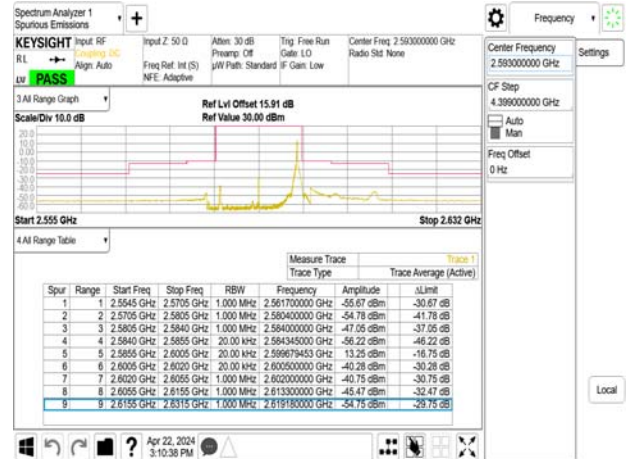
Emission Mask_Band41_15MHz_OPSK_RB1_74_CH40620
