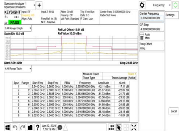
Emission Mask_Band38_20MHz_QPSK_RB100_0_CH38000
