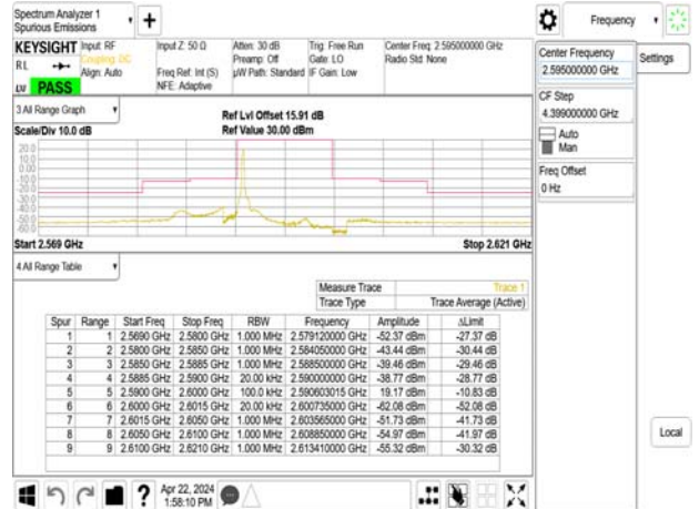
Emission Mask_Band38_10MHz_QPSK_RB1_0_CH38000
