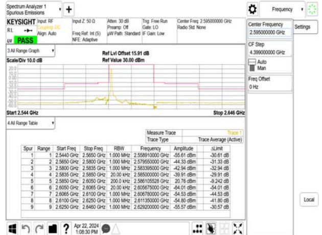
Emission Mask_Band38_20MHz_OPK RB1_0_CH38000
