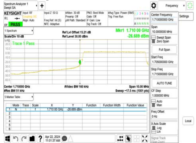
Band Edge_Band66_5MHz_QPSK_RB25_0_CH131997
