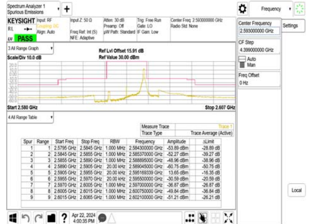
Emission Mask_Band41_5MHz_QPSK_RB1_24_CH40620
