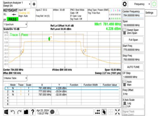
Band13_10MHz_OPSK_RB1_0_CH23230
