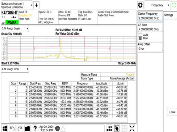
Emission Mask_Band38_15MHz_OPSK_RB1_0_CH38000
