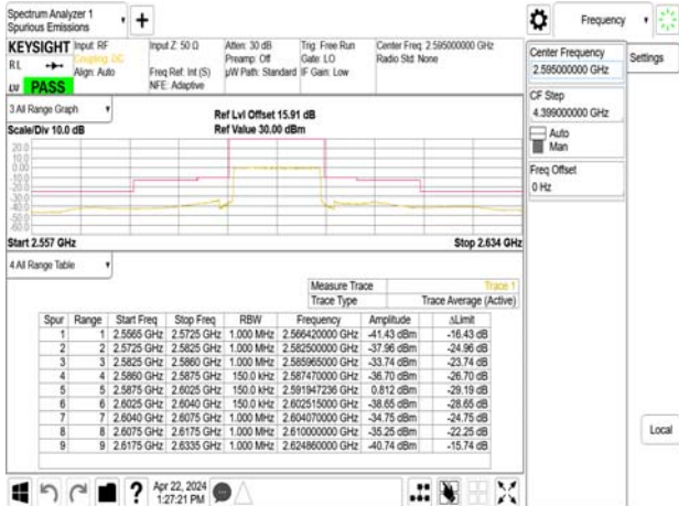
Emission Mask_Band38_15MHz_OPK RB75_0_CH38000
