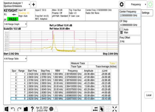
Emission Mask_Band41_20MHz_OPSK_RB1_0_CH40620
