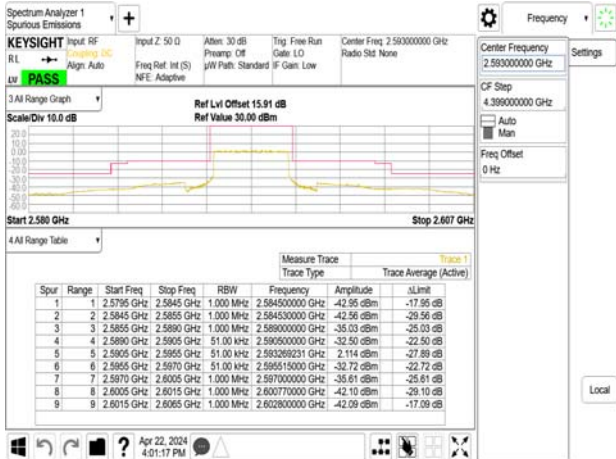
Emission Mask_Band41_5MHz_QPSK_RB25_0_CH40620
