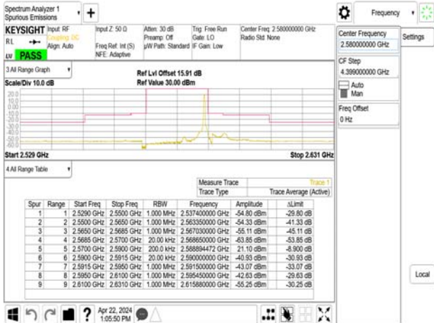
Emission Mask_Band38_20MHz_QPSK_RB1_99_CH38000
