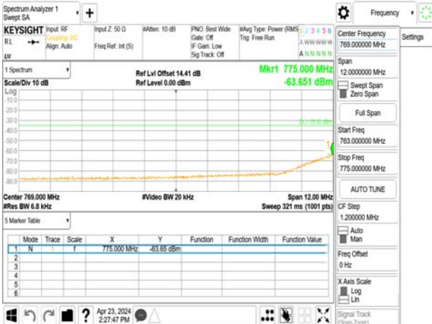
Band13_5MHz_QPSK_RB25_0_CH23205
