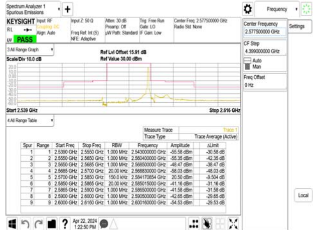
Emission Mask_Band38_15MHz_OPSK_RB1_74_CH38000
