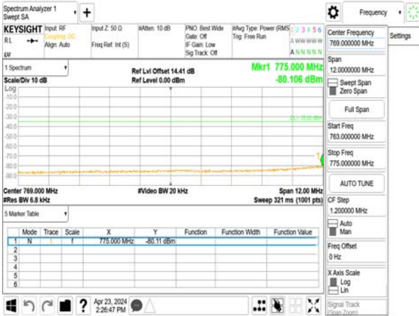
Band13_5MHz_QPSK_RB1_24_CH23255
