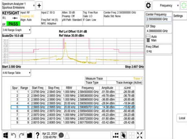
Emission Mask_Band41_5MHz_QPSK_RB1_0_CH40620
