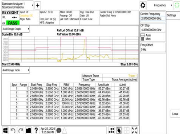
Emission Mask_Band38_10MHz_QPSK_RB1_49_CH38000
