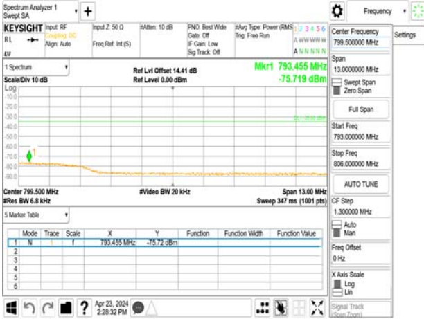
Band Edge_Band13_10MHz_OPSK_RB1_0_CH23230
