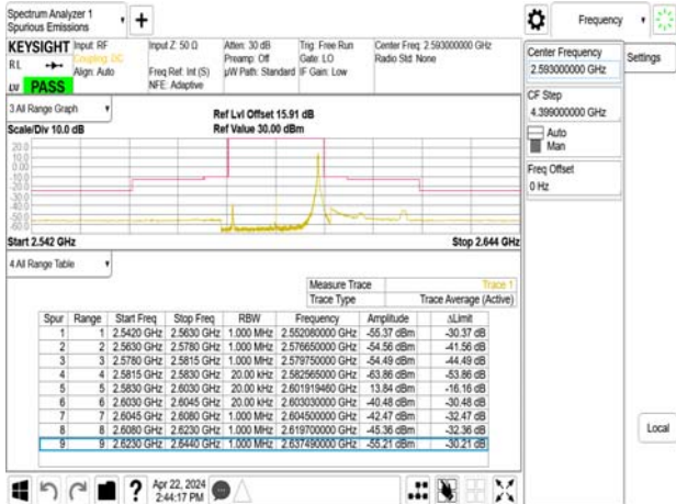
Emission Mask_Band41_20MHz_QPSK_RB1_99_CH40620
