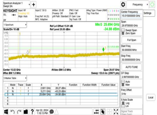
Band41_20MHz_QPSK_RB1_0_CH39750
