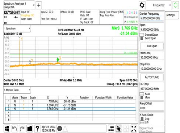
Band17_10MHz_QPSK_RB1_0_CH23780
