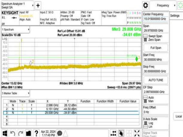
Band38_20MHz_QPSK_RB1_0_CH38000
