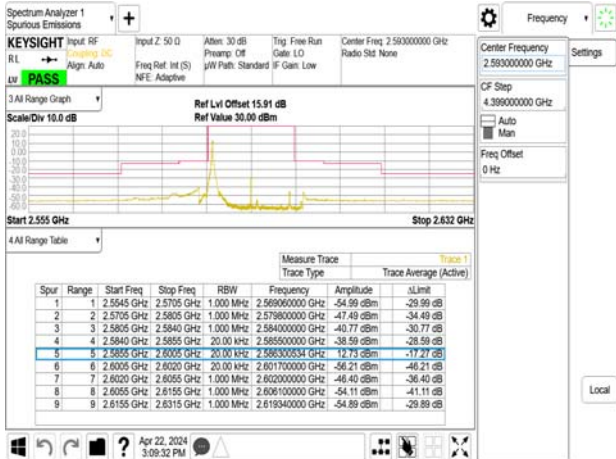
Emission Mask_Band41_15MHz_OPSK_RB1_0_CH40620
