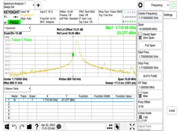
Band Edge_Band66_5MHz_QPSK_RB1_24_CH132647
