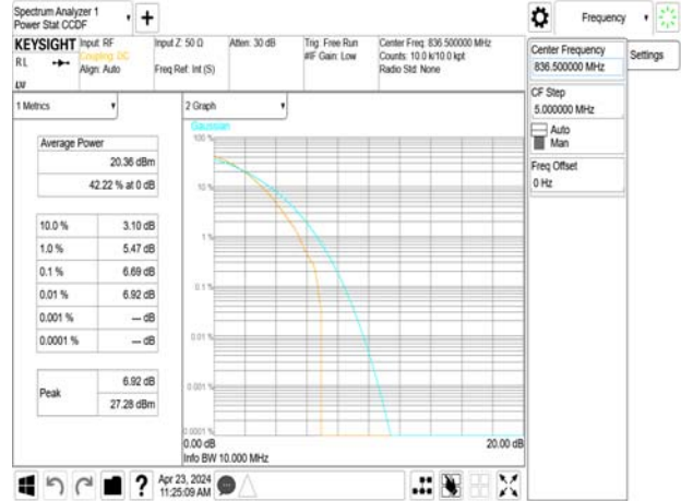
Band5_10MHz_64QAM_RB50_0_CH20600
