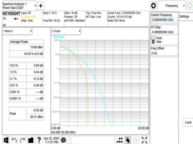
Band38_20MHz_64QAM_RB100_0_CH38000
