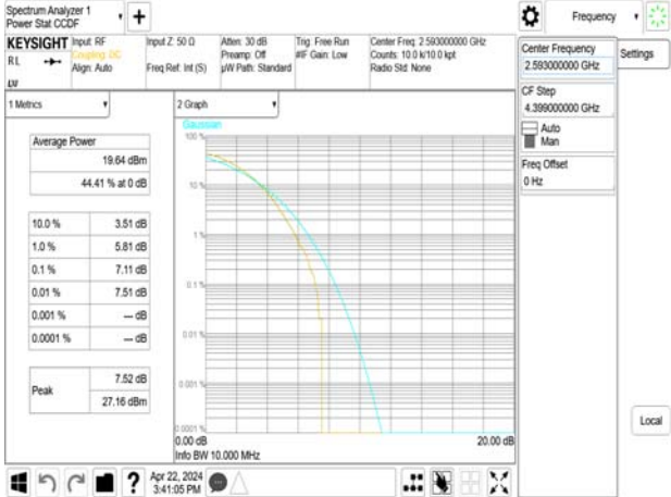
Band41_10MHz_64QAM_RB50_0_CH40620
