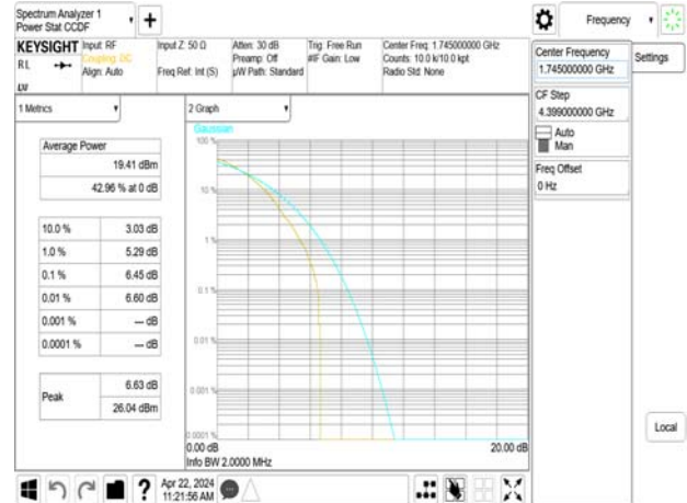
Band66_1.4MHz_64QAM_RB6_0_CH132322
