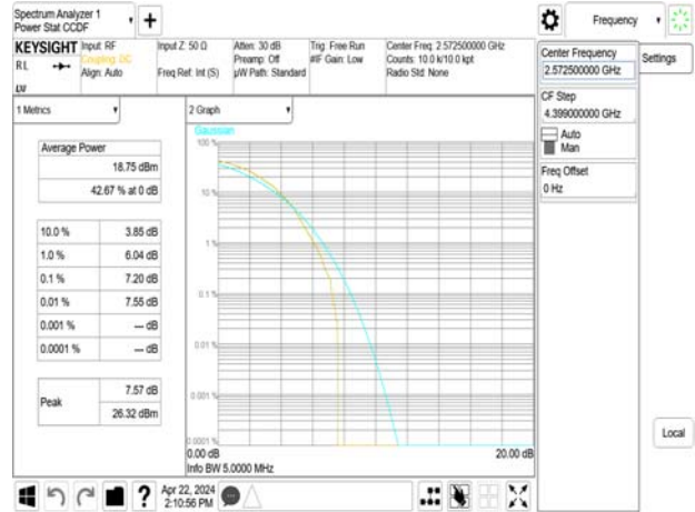
Band38_5MHz_64QAM_RB25_0_CH38000
