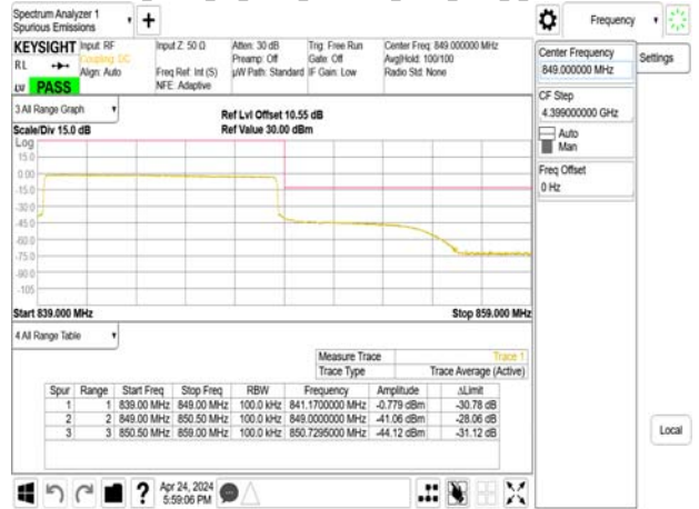
Band5_15MHz_DFT_s_OFDM_SCS15kHz_BPSK_RB1_0_CH166300
