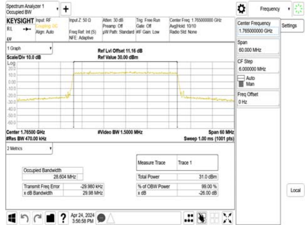
Band66_30MHz_DFT_s_OFDM_SCS15kHz_QPSK_RB160_0_CH353000
