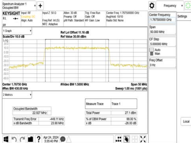
Band66_25MHz_DFT_s_OFDM_SCS15kHz_OPSK_RB128_0_CH353500
