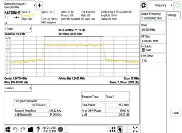
Band66_25MHz_DFT_s_OFDM_SCS15kHz_16QAM_RB128_0_CH353500
