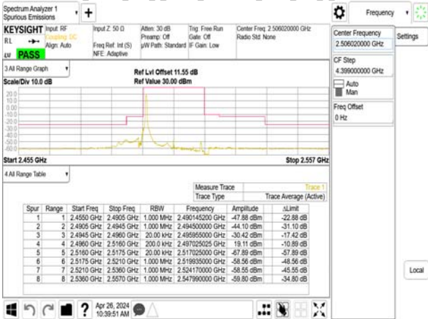
Band41_20MHz_DFT_s_OFDM_SCS30kHz_BPSK_RB1_0_CH501204
