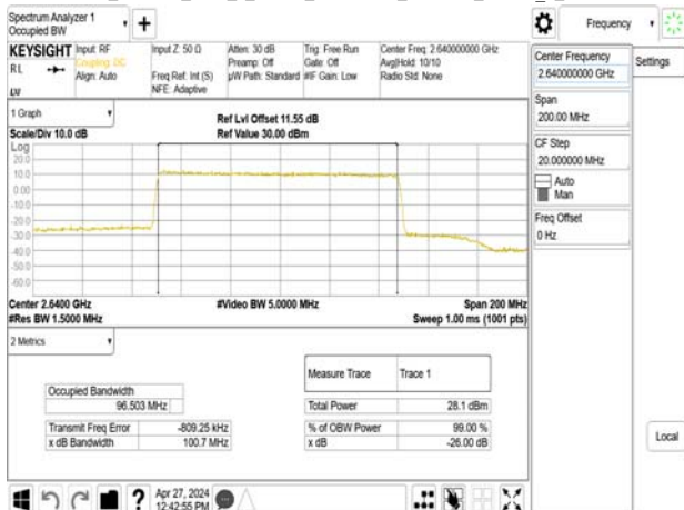
Band41_100MHz_DFT_s_OFDM_SCS30kHz_256QAM_RB270_0_CH528000
