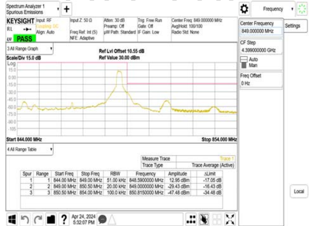
Band5_5MHz_CP_OFDM_SCS15kHz_QPSK_RB1_24_CH169300
