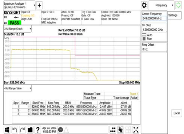
Band5_20MHz_CP_OFDM_SCS15kHz_QPSK_RB1_0_CH166800
