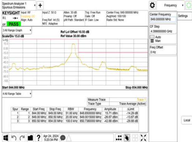
Band5_5MHz_DFT_s_OFDM_SCS15kHz_BPSK_RB25_0_CH165300
