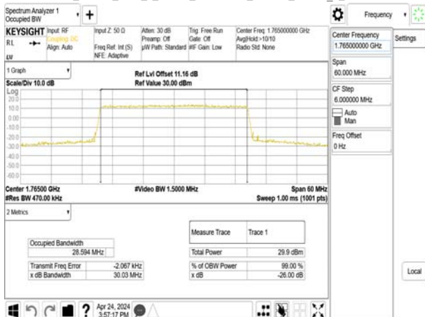
Band66_30MHz_DFT_s_OFDM_SCS15kHz_16QAM_RB160_0_CH353000
