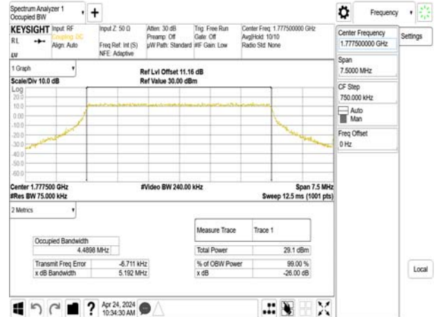
Band66_5MHz_DFT_s_OFDM_SCS15kHz_16QAM_RB25_0_CH355500
