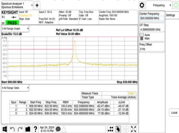
Band5_15MHz_CP_OFDM_SCS15kHz_QPSK_RB1_0_CH166300
