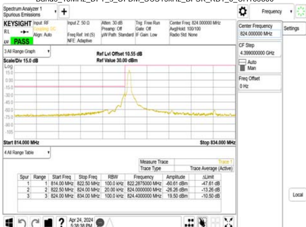
Band5_10MHz_DFT_s_OFDM_SCS15kHz_BPSK_RB1_0_CH165800
