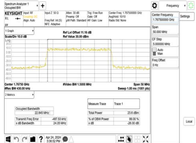
Band66_25MHz_DFT_s_OFDM_SCS15kHz_256QAM_RB128_0_CH353500
