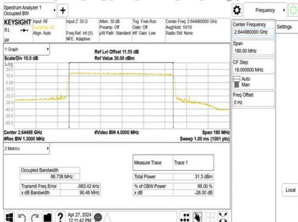
Band41_90MHz_DFT_s_OFDM_SCS30kHz_QPSK_RB243_0_CH528996
