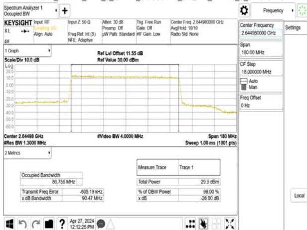
Band41_90MHz_DFT_s_OFDM_SCS30kHz_64QAM_RB243_0_CH528996
