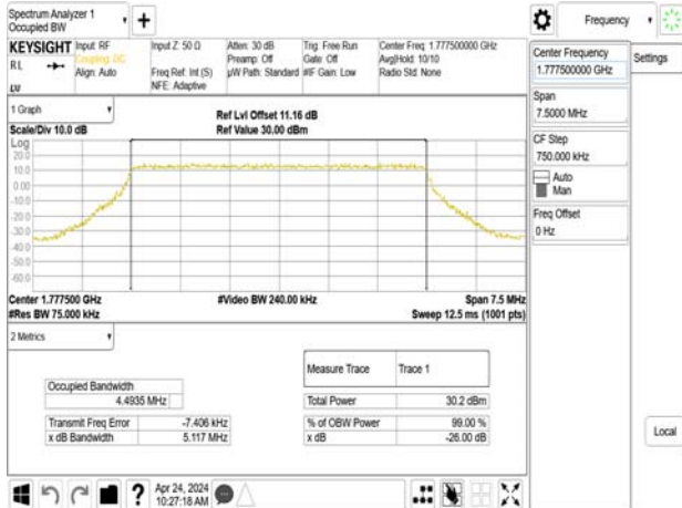
Band66_5MHz_DFT_s_OFDM_SCS15kHz_OPSK_RB25_0_CH355500
