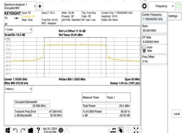
Band66_30MHz_DFT_s_OFDM_SCS15kHz_64QAM_RB160_0_CH353000
