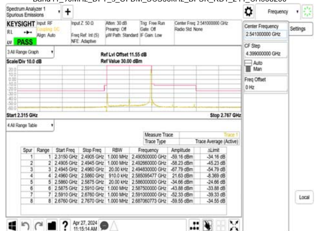
Band41_90MHz_DFT_s_OFDM_SCS30kHz_BPSK_RB1_244_CH508200
