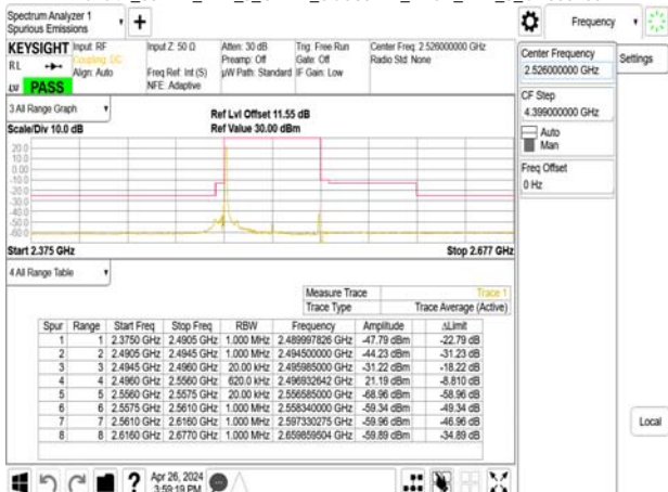
Band41_60MHz_DFT_s_OFDM_SCS30kHz_BPSK_RB1_0_CH505200
