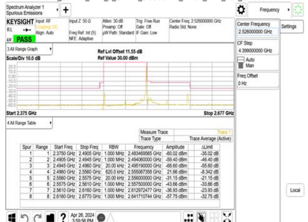
Band41_60MHz_DFT_s_OFDM_SCS30kHz_BPSK_RB1_161_CH505200
