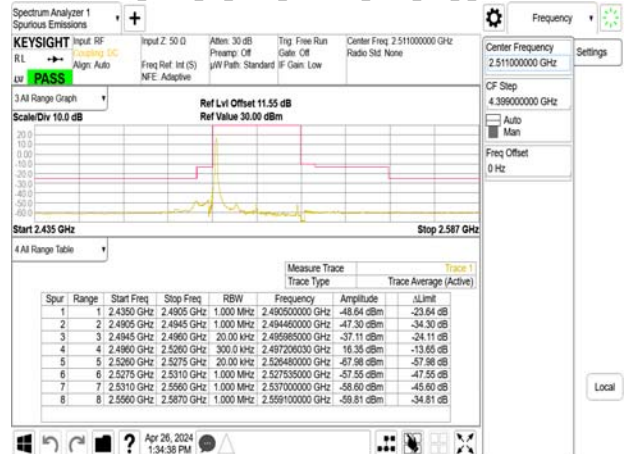
Band41_30MHz_CP_OFDM_SCS30kHz_QPSK_RB1_0_CH502200
