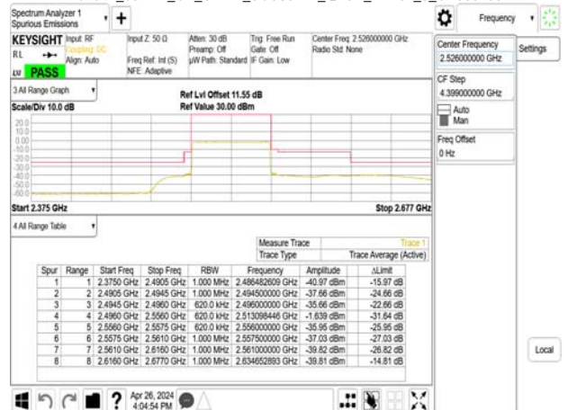
Band41_60MHz_CP_OFDM_SCS30kHz_QPSK_RB162_0_CH505200
