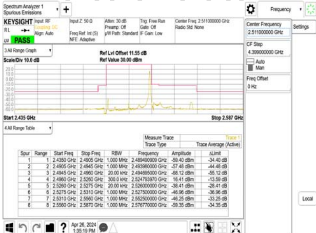
Band41_30MHz_CP_OFDM_SCS30kHz_QPSK_RB1_77_CH502200
