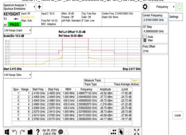
Band41_40MHz_CP_OFDM_SCS30kHz_QPSK_RB106_0_CH503202
