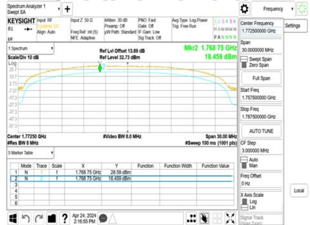
Band66_15MHz_DFT_s_OFDM_SCS15kHz_256QAM_RB75_0_CH354500
