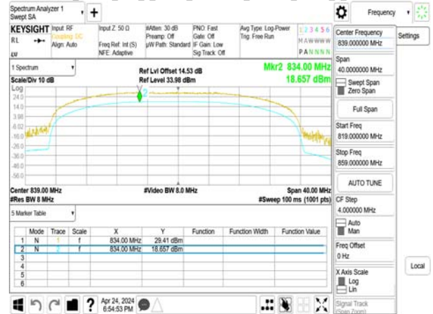
Band5_20MHz_DFT_s_OFDM_SCS15kHz_256QAM_RB100_0_CH167800
