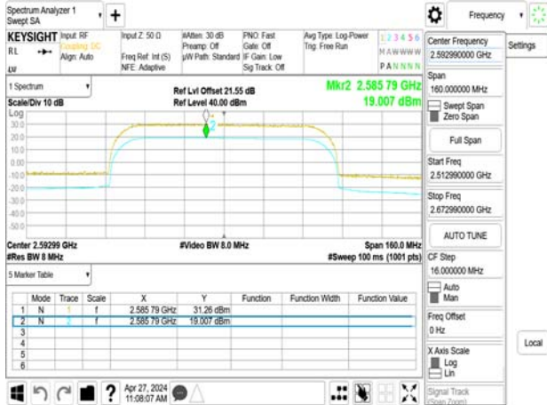
Band41_80MHz_DFT_s_OFDM_SCS30kHz_256QAM_RB216_0_CH529998
