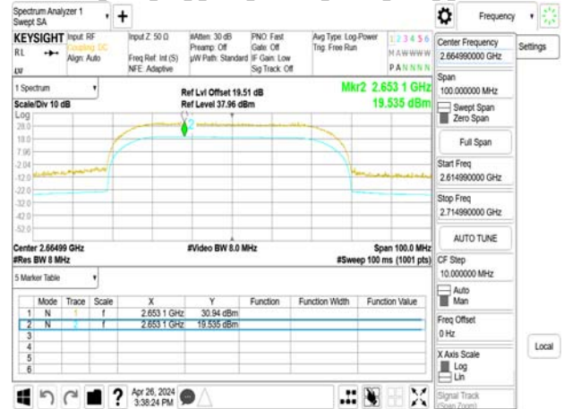
Band41_50MHz_DFT_s_OFDM_SCS30kHz_256QAM_RB128_0_CH532998
