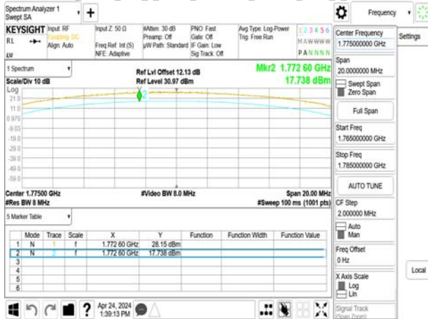
Band66_10MHz_DFT_s_OFDM_SCS15kHz_256QAM_RB50_0_CH355000
