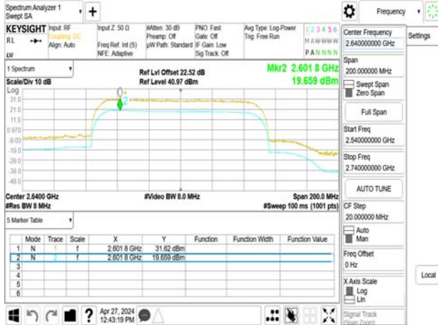
Band41_100MHz_DFT_s_OFDM_SCS30kHz_256QAM_RB270_0_CH528000
