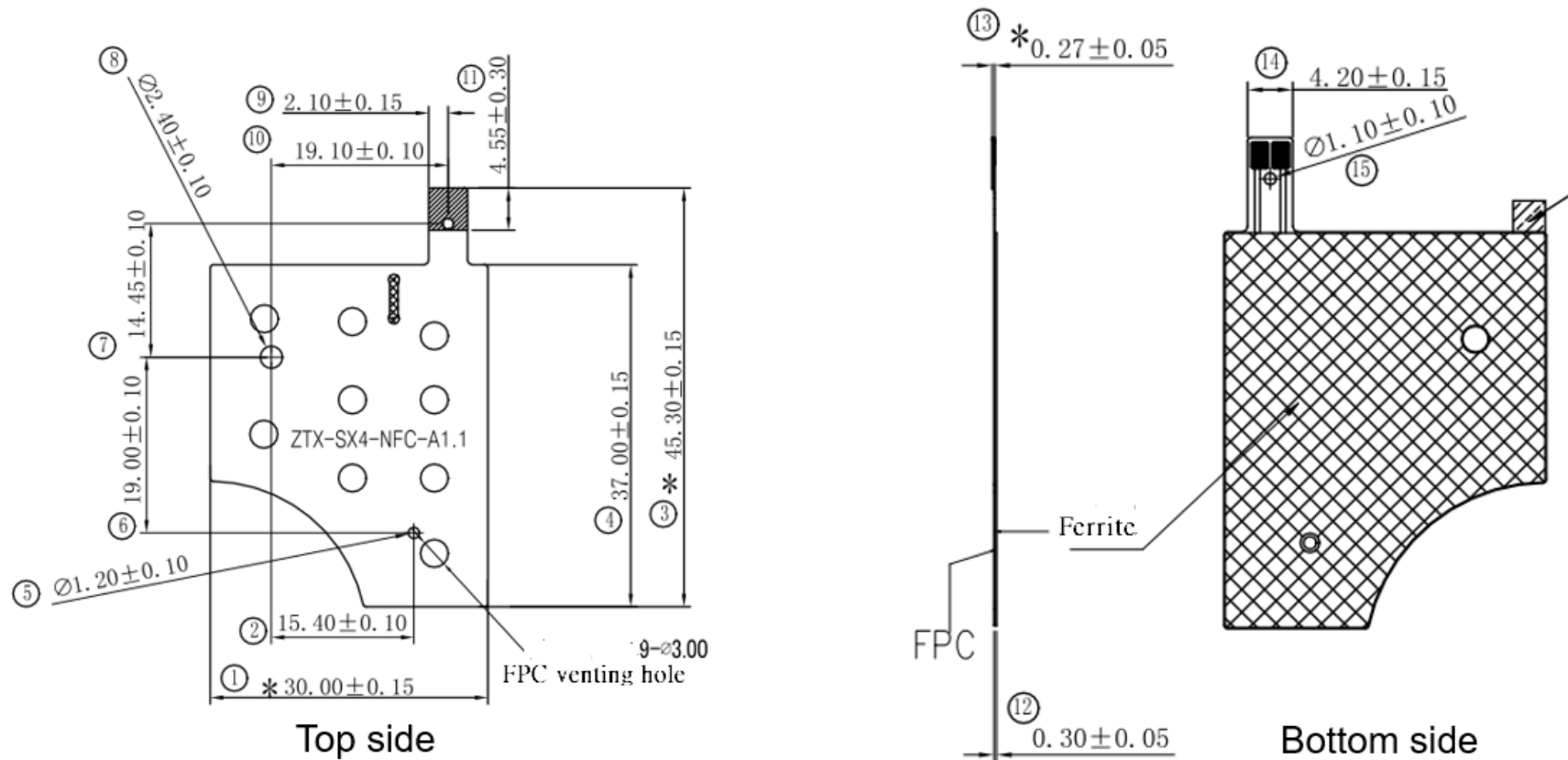
Antenna: Dimensions (unit: mm)
