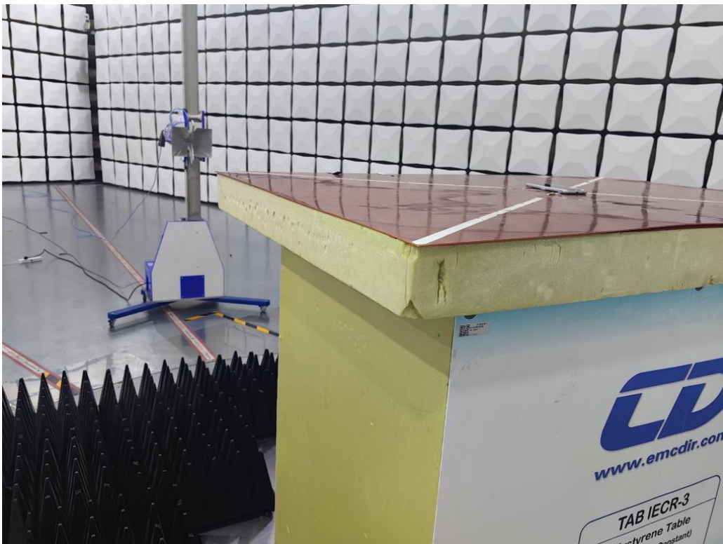
RE >1GHz
