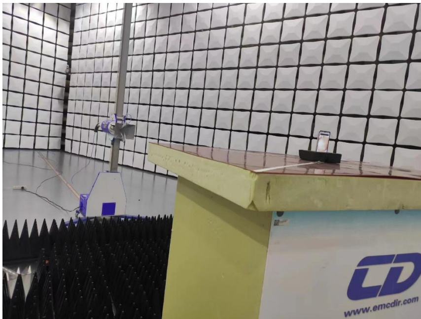
RE >1GHz
