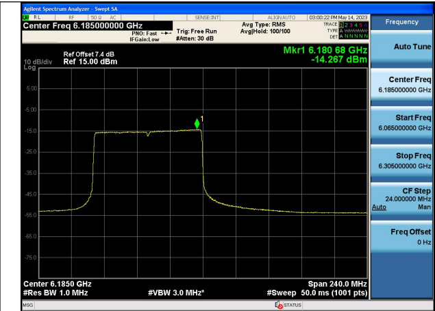
Mode:802.11ax HE160 Tone:996T Frequency:6185MHz Chain0
