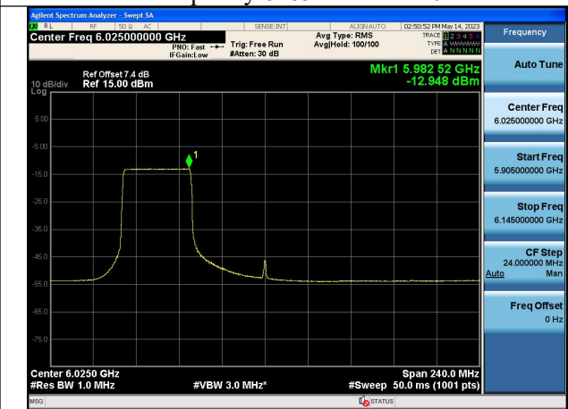
Mode:802.11ax HE160 Tone:484T Frequency:6025MHz Chain1
