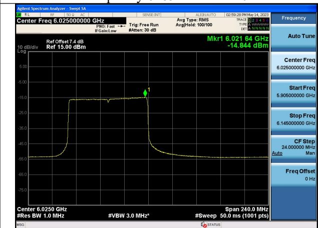
Mode:802.11ax HE160 Tone:996T Frequency:6025MHz Chain1
