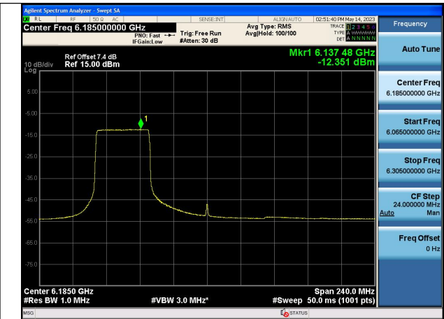
Mode:802.11ax HE160 Tone:484T Frequency:6185MHz Chain0
