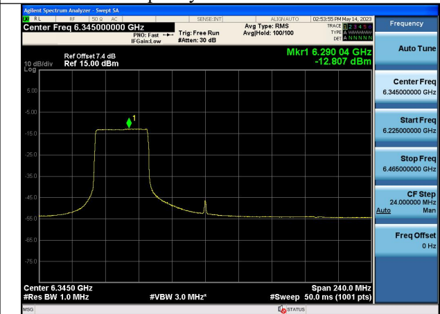
Mode:802.11ax HE160 Tone:484T Frequency:6345MHz Chain1
