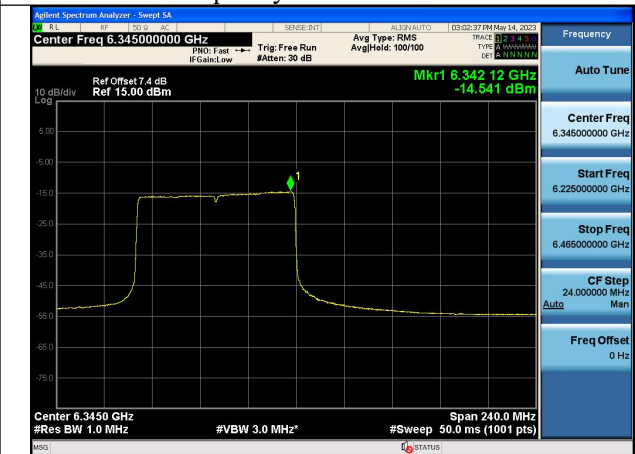
Mode:802.11ax HE160 Tone:996T Frequency:6345MHz Chain1
