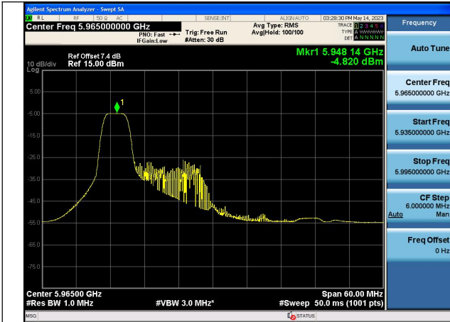
Mode:802.11ax HE40 Tone:52T Frequency:5965MHz Chain0
