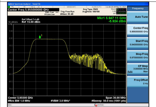
Mode:802.11ax HE20 Tone:106T Frequency:5955MHz Chain1
