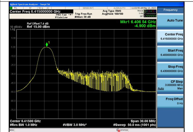
Mode:802.11ax HE20 Tone:26T Frequency:6415MHz Chain1
