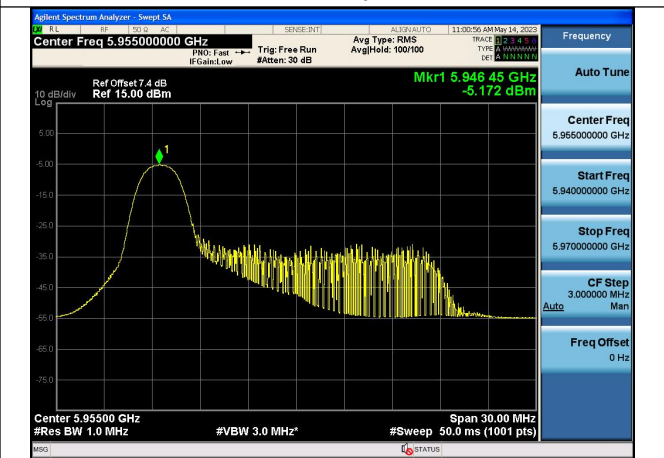
Mode:802.11ax HE20 Tone:26T Frequency:5955MHz Chain1
