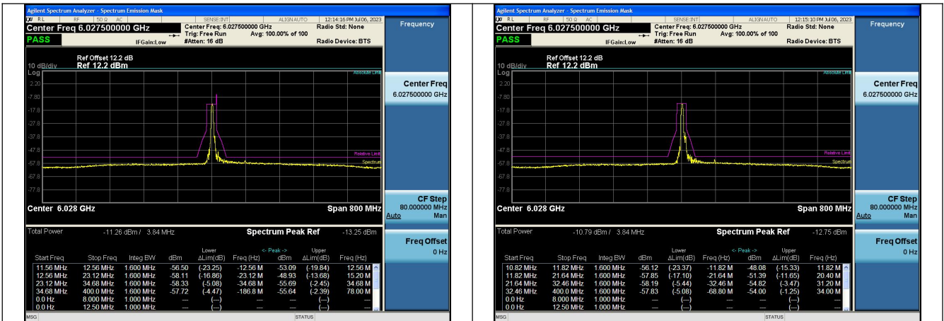
Test Mode:802.11ax HE160 6025MHz Tone:52T Chain0
