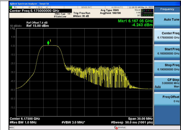
Mode:802.11ax HE20 Tone:52T Frequency:6175MHz Chain0
