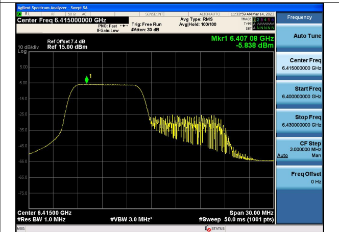
Mode:802.11ax HE20 Tone:106T Frequency:6415MHz Chain1
