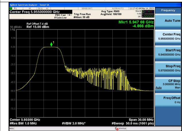
Mode:802.11ax HE20 Tone:52T Frequency:5955MHz Chain1
