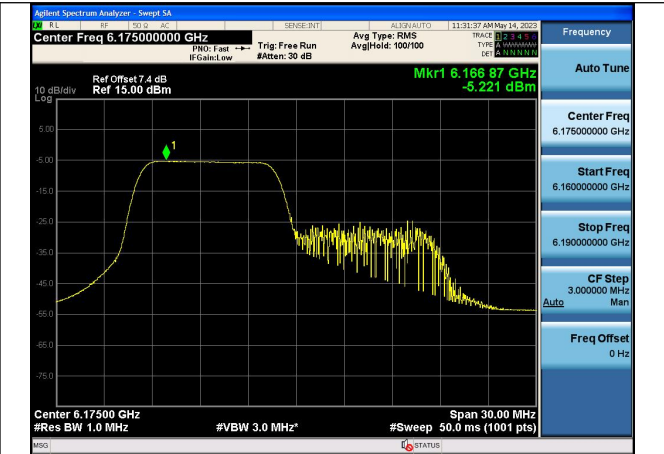
Mode:802.11ax HE20 Tone:106T Frequency:6175MHz Chain0
