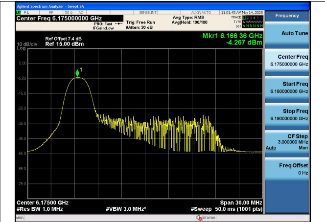
Mode:802.11ax HE20 Tone:26T Frequency:6175MHz Chain0
