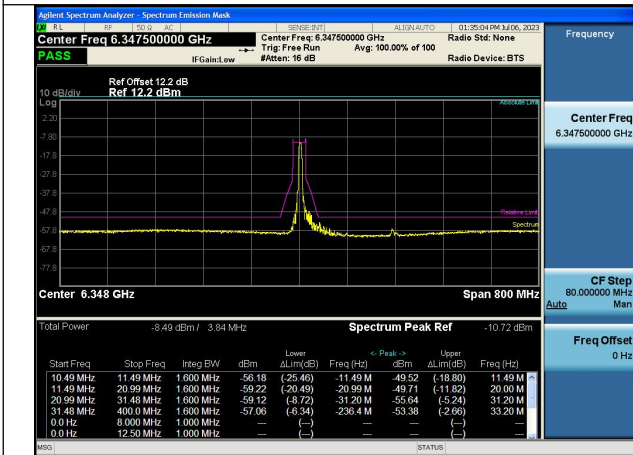
Test Mode:802.11ax HE160 6345MHz Tone:52T Chain0
