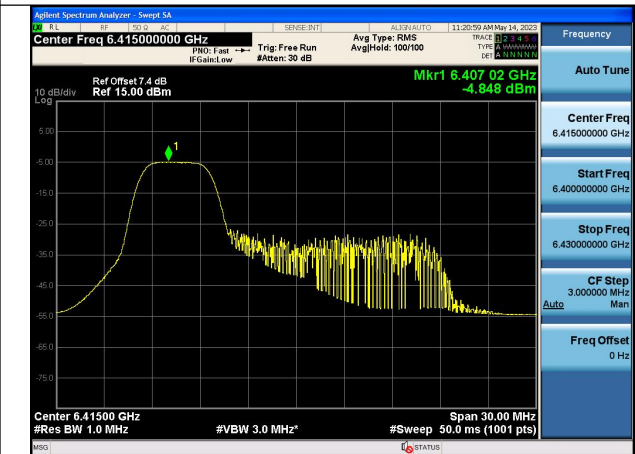
Mode:802.11ax HE20 Tone:52T Frequency:6415MHz Chain1
