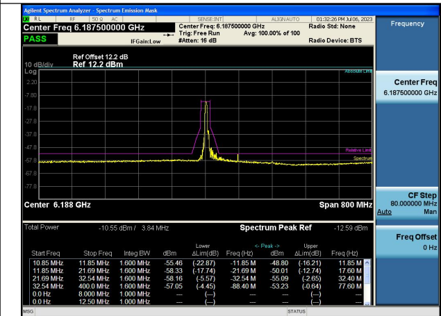
Test Mode:802.11ax HE160 6185MHz Tone:52T Chain1
