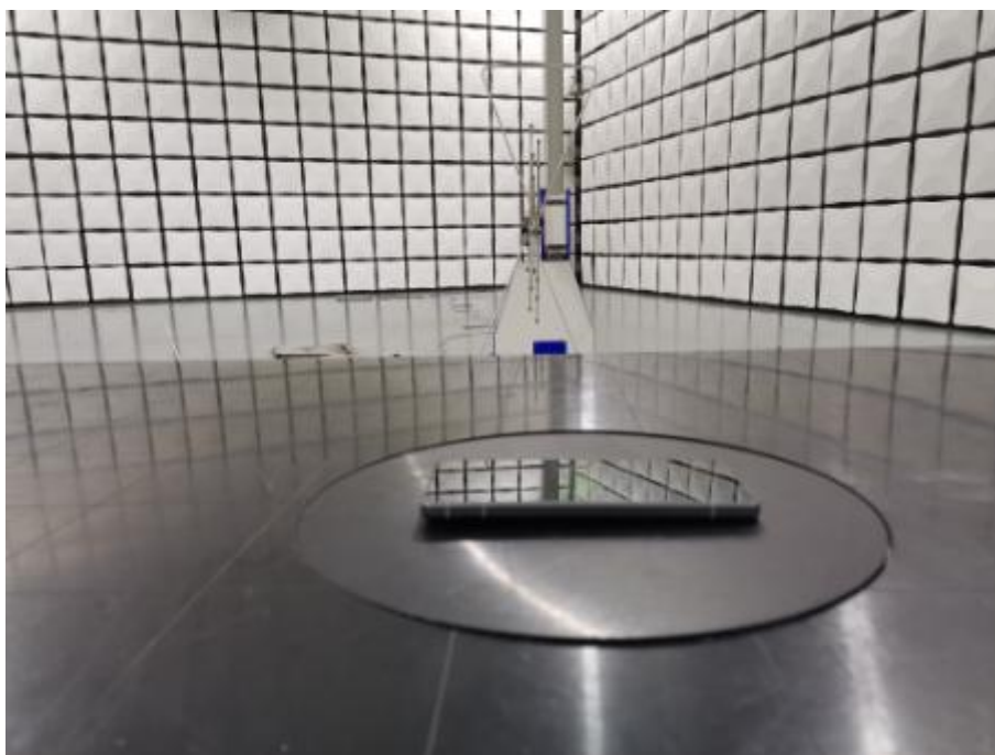
30MHz-1GHz Vertical
