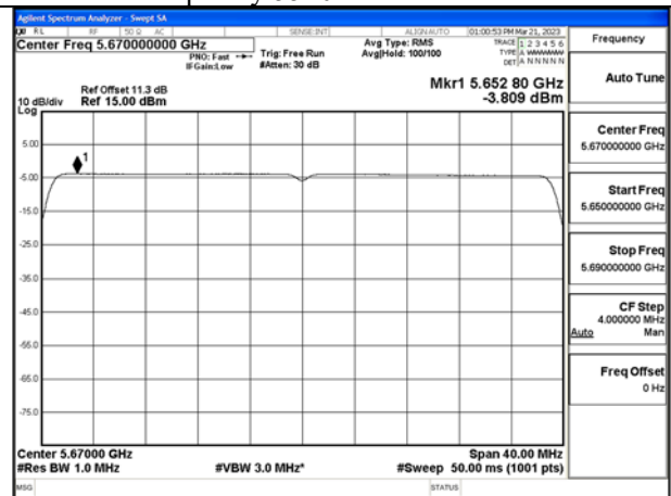
Mode:802.11ax HE40 Tone:484T Frequency:5670MHz Ant:Chain1
