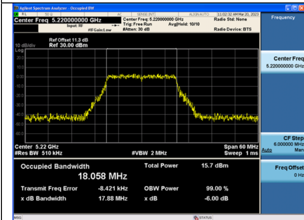
Test Mode:802.11n HT20 5220MHz Chain1
