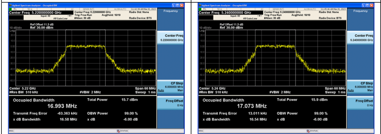
Test Mode:802.11a 5220MHz Chain1
