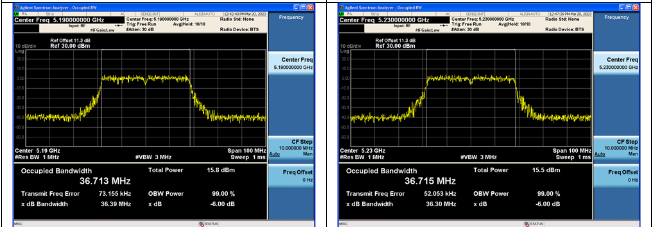
Test Mode:802.11n HT40 5190MHz Chain1
